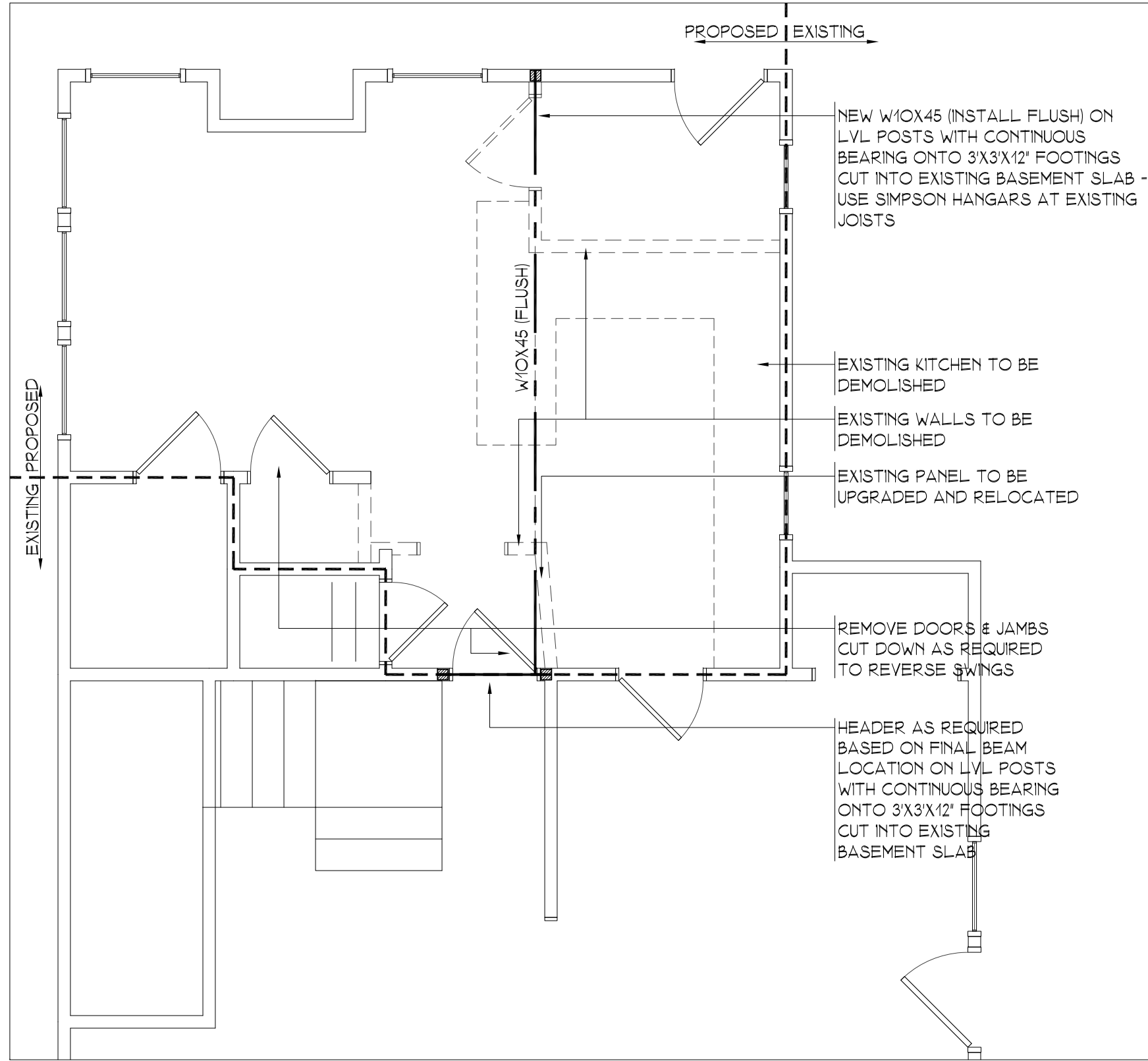
DEMO & STRUCTURAL PLAN SCALE: 1/4" = 1'-0"
