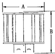
3-8" High Wind Vent Top
