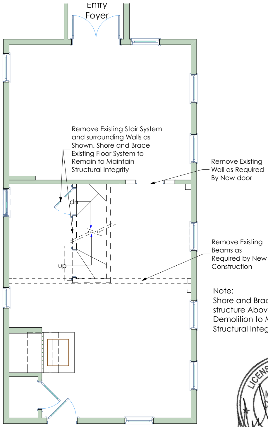
Partial First Floor Demolition Plan SCALE: 3/16" = 1'-0"
