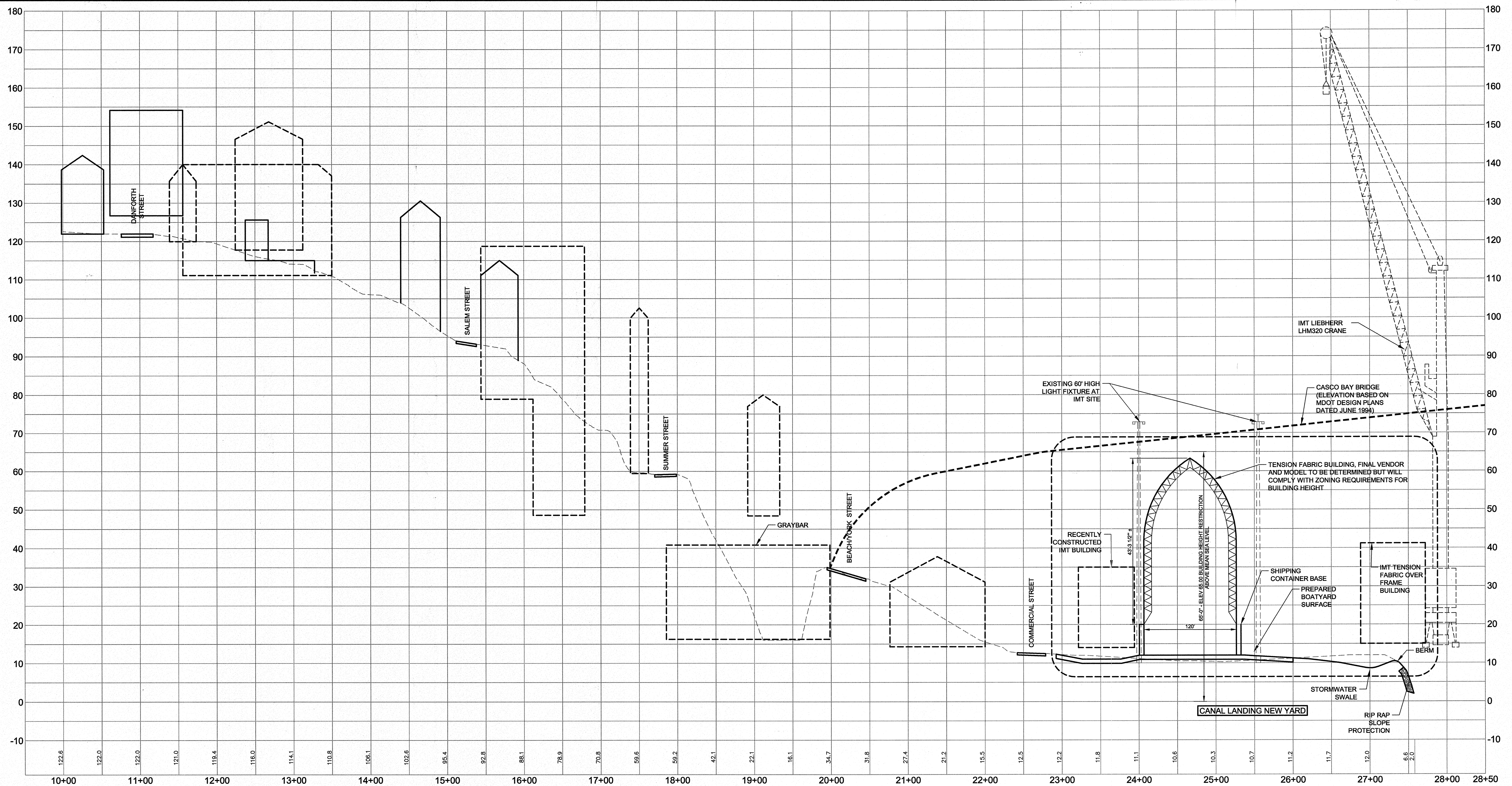
THE NEIGHBORHOOD SECTION SCALE: 1"= 60' HORIZ., 1"= 12' VERT.
