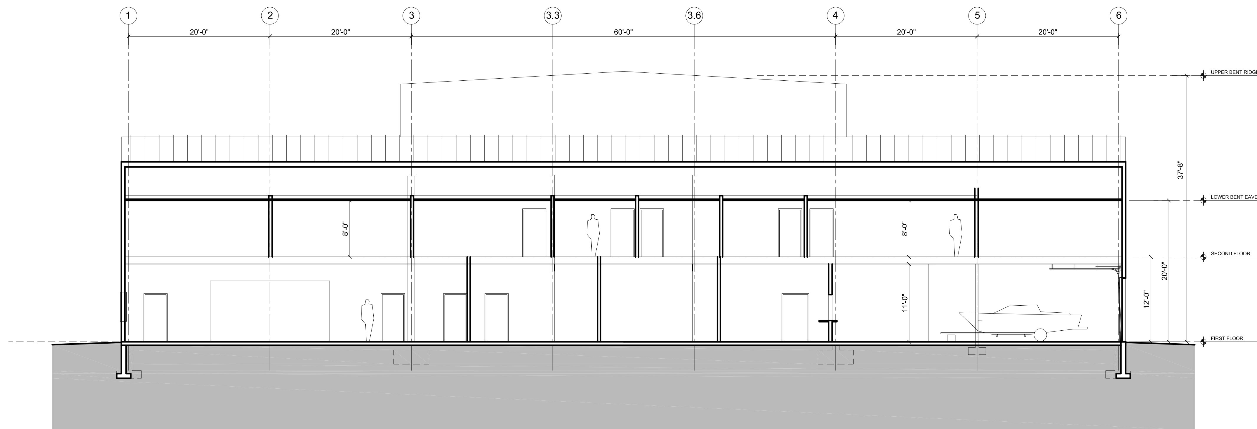
SECTION (B-B) AT ADMINISTRATION / RETAIL SCALE 1/8"=1'-0"
