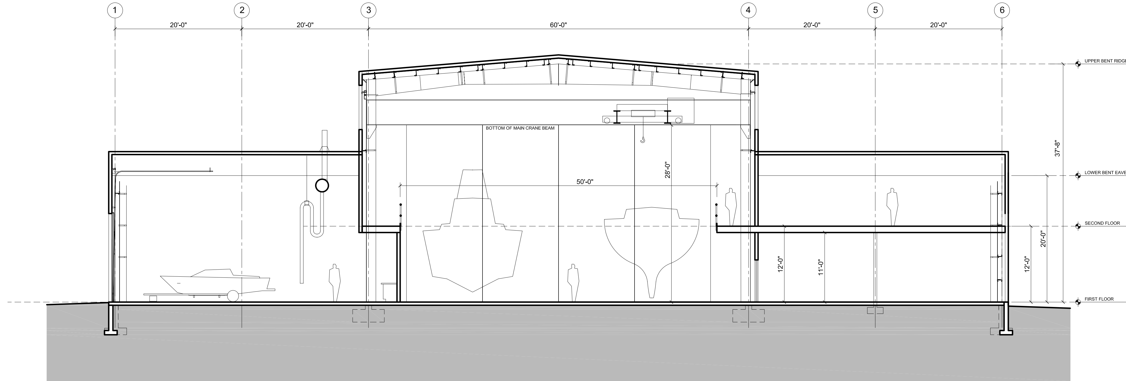
SECTION (A-A) AT CLERESTORY SCALE 1/8"=1'-0"
