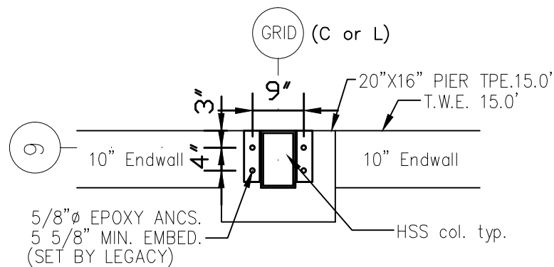
G Baseplate G 1/2"=1'-0"
