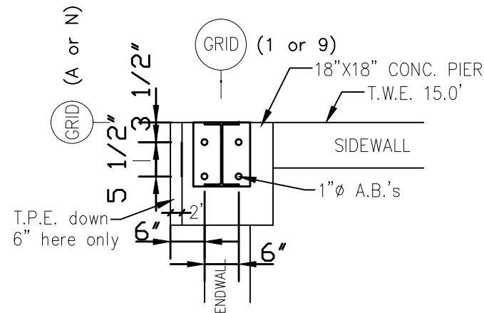
A Baseplate A 1/2"=1'-0"
