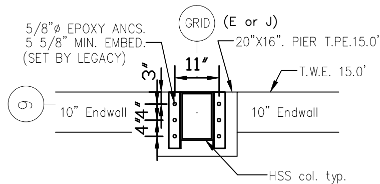
H Baseplate H 1/2"=1'-0"
