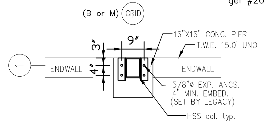
C Baseplate C 1/2"=1'-0"
