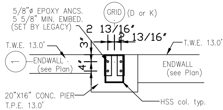
D Baseplate D 1/2"=1'-0"
