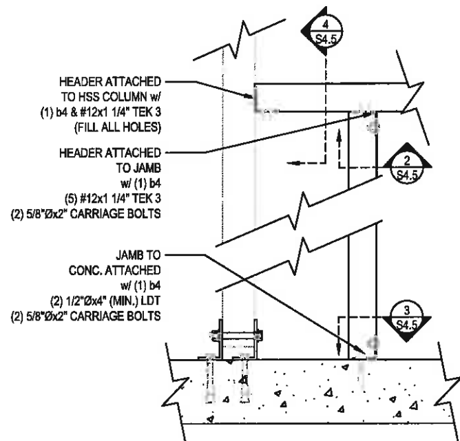
1 8C14 DOOR FRAME DETAIL SCALE: 3/4" = 1'-0"
