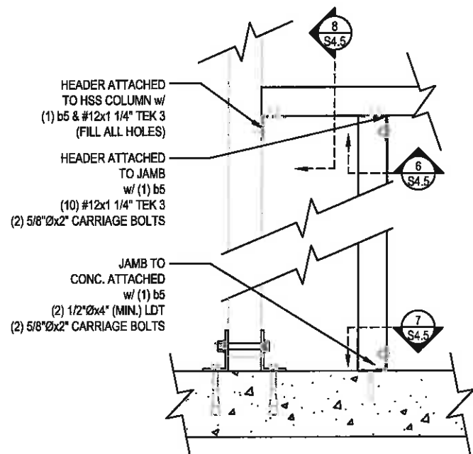
5 12C12 DOOR FRAME DETAIL SCALE: 3/4" = 1'-0"
