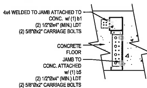
7 12C12 JAMB TO CONCRETE SCALE: 3/4" = 1'-0"
