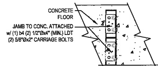
3 8C14 JAMB TO CONCRETE SCALE: 3/4" = 1'-0"
