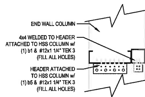
8 12C12 TO COLUMN SECTION SCALE: 3/4" = 1'-0"
