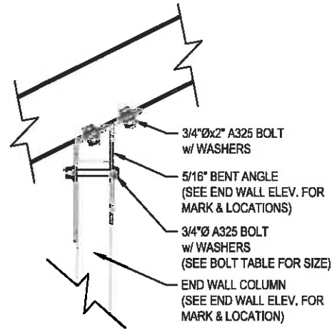
1 COLUMN TOP ATTACHMENT SCALE: 3/4" = 1'-0"
