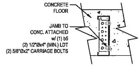
6 12C12 JAMB TO CONCRETE SCALE: 3/4" = 1'-0"
