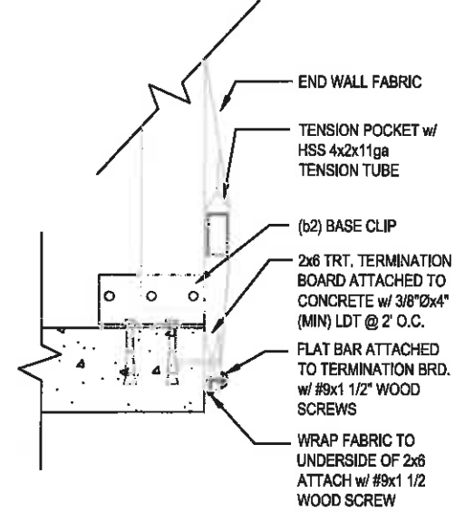
3 END WALL TERMINATION SCALE: 3/4" = 1'-0"
