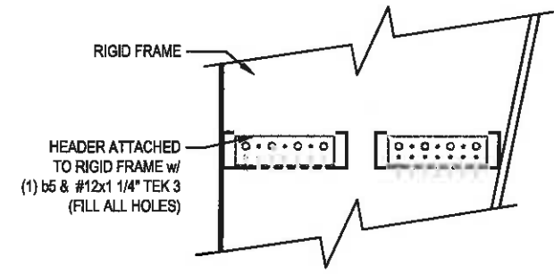
7 12C12 TO RIGID FRAME SCALE: 3/4" = 1'-0"
