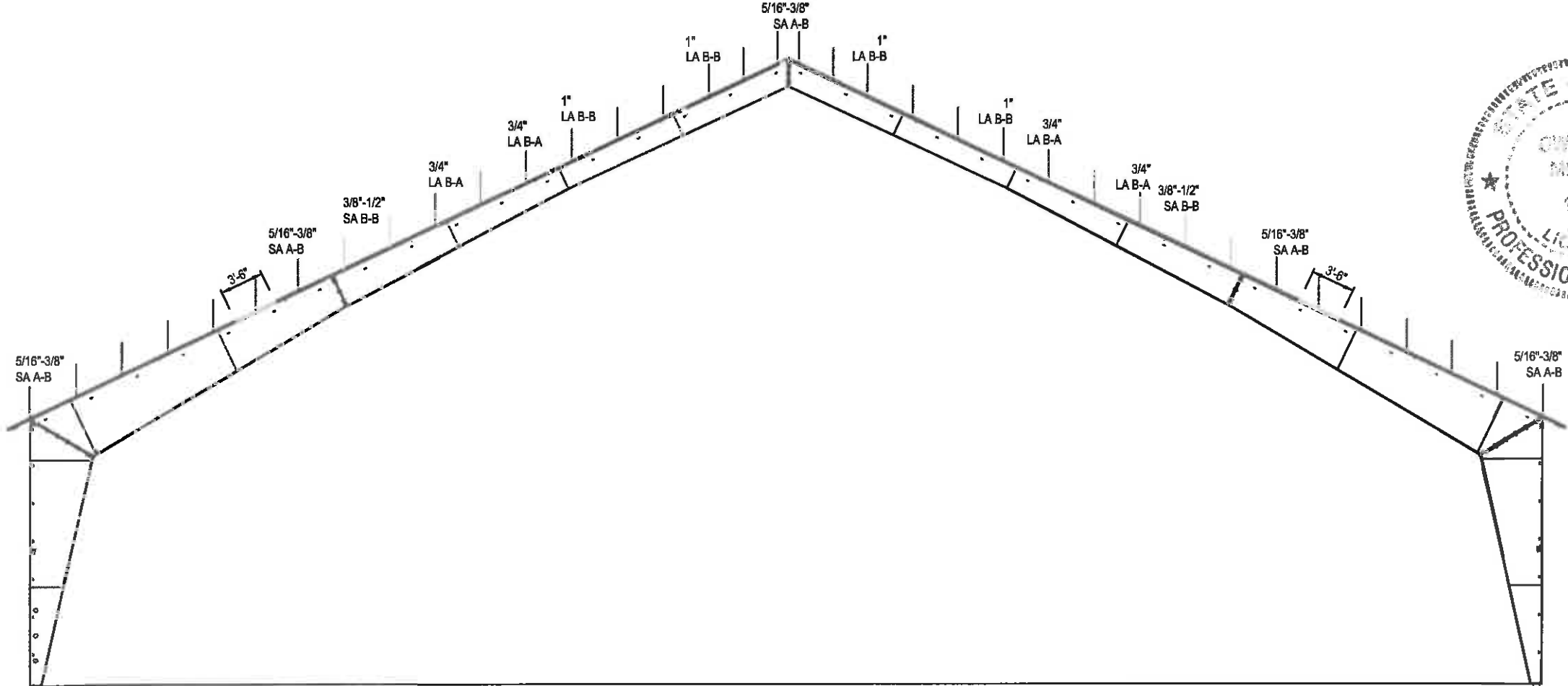
1 EXTRUSION LAYOUT COMMON FRAMES
