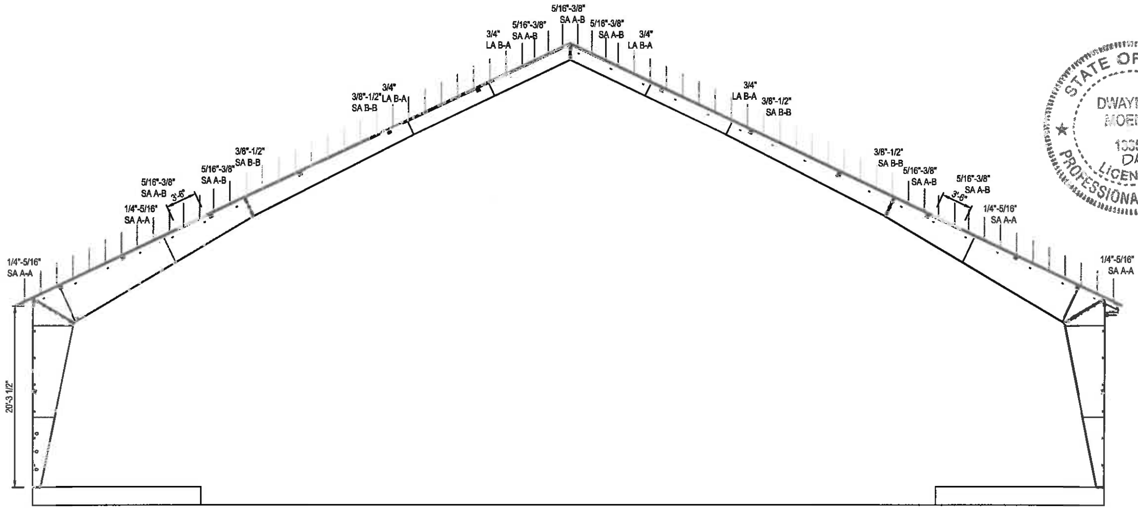
1 EXTRUSION LAYOUT FRAME LINE 1
