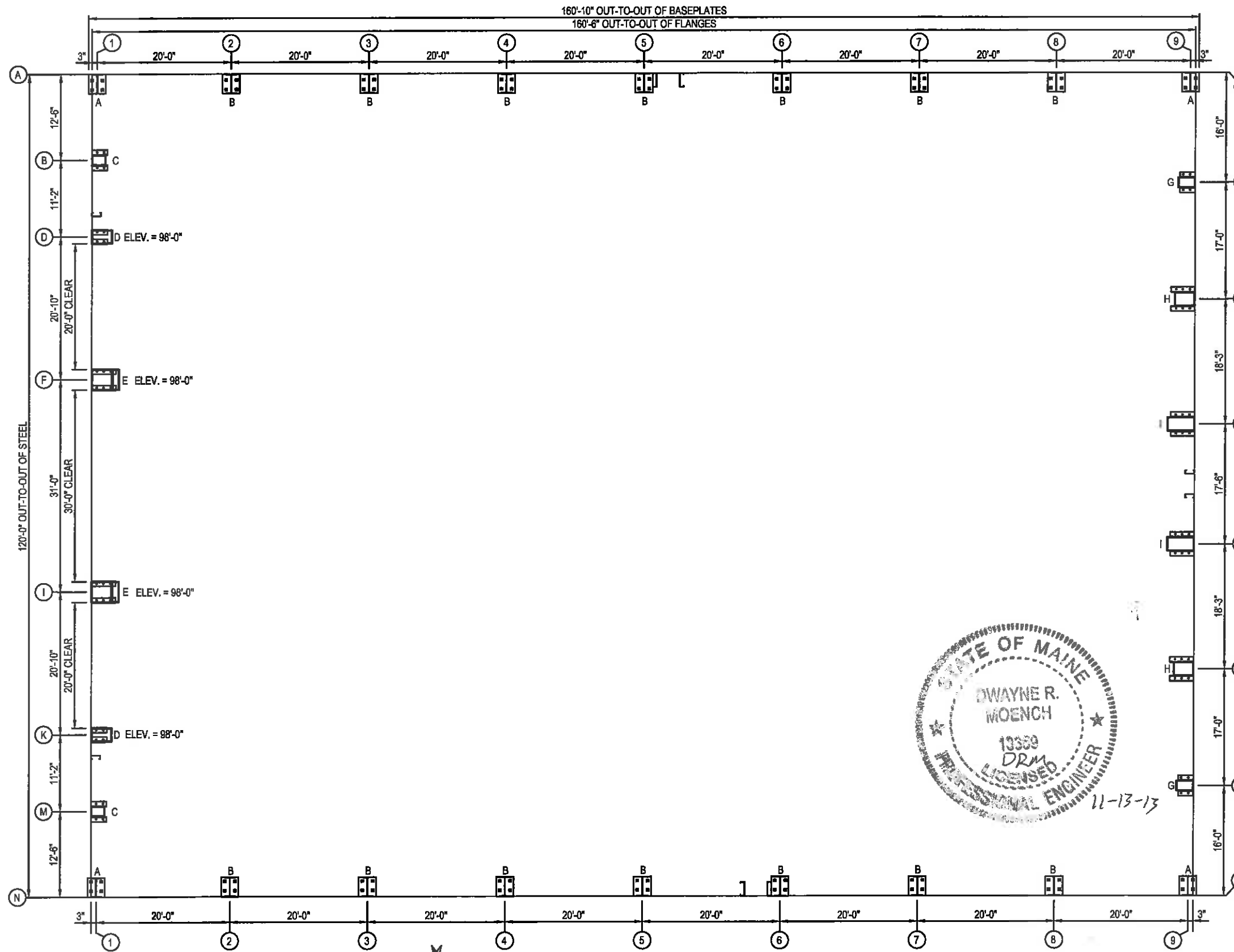
1 BASEPLATE LAYOUT ALL BASEPLATES @ ELEV. 100'-0" U.N.O.
