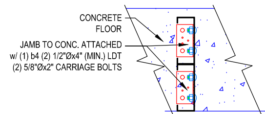
3 8C14 JAMB TO CONCRETE SCALE: 3/4" = 1'-0"
