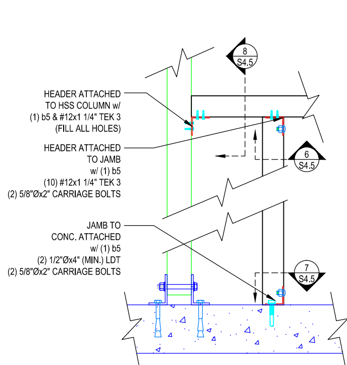
5 12C12 DOOR FRAME DETAIL SCALE: 3/4" = 1'-0"
