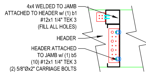
6 12C12 HEADER TO JAMB SCALE: 3/4" = 1'-0"
