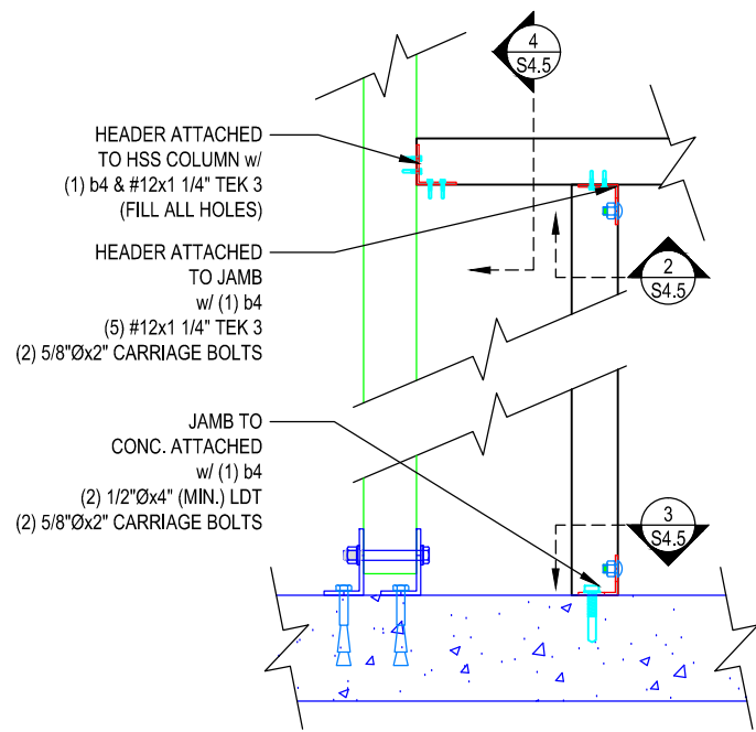
1 8C14 DOOR FRAME DETAIL SCALE: 3/4" = 1'-0"
