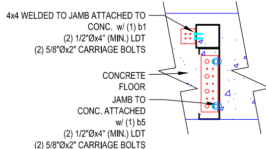
7 12C12 JAMB TO CONCRETE SCALE: 3/4" = 1'-0"
