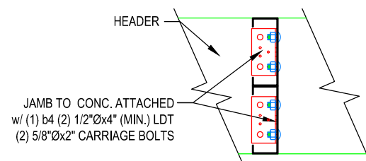
2 8C14 HEADER TO JAMB SCALE: 3/4" = 1'-0"
