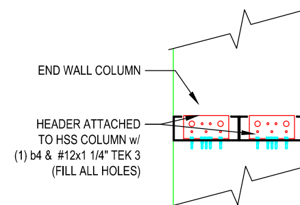
4 8C14 TO COLUMN SECTION SCALE: 3/4" = 1'-0"
