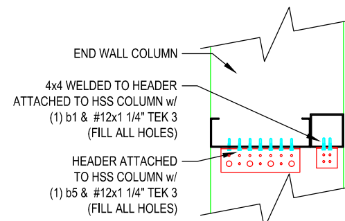
8 12C12 TO COLUMN SECTION SCALE: 3/4" = 1'-0"
