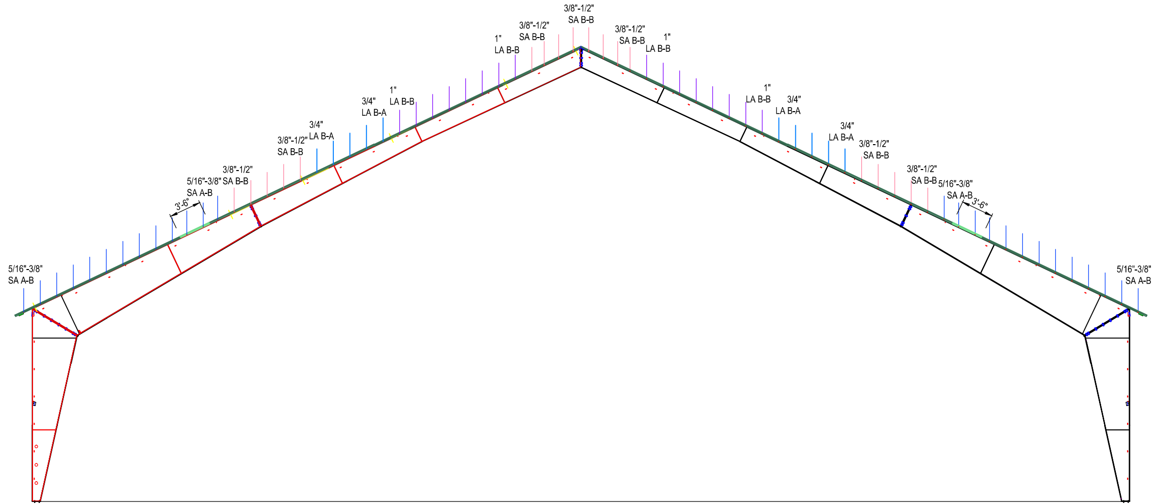
1 EXTRUSION LAYOUT FRAME LINE 9
