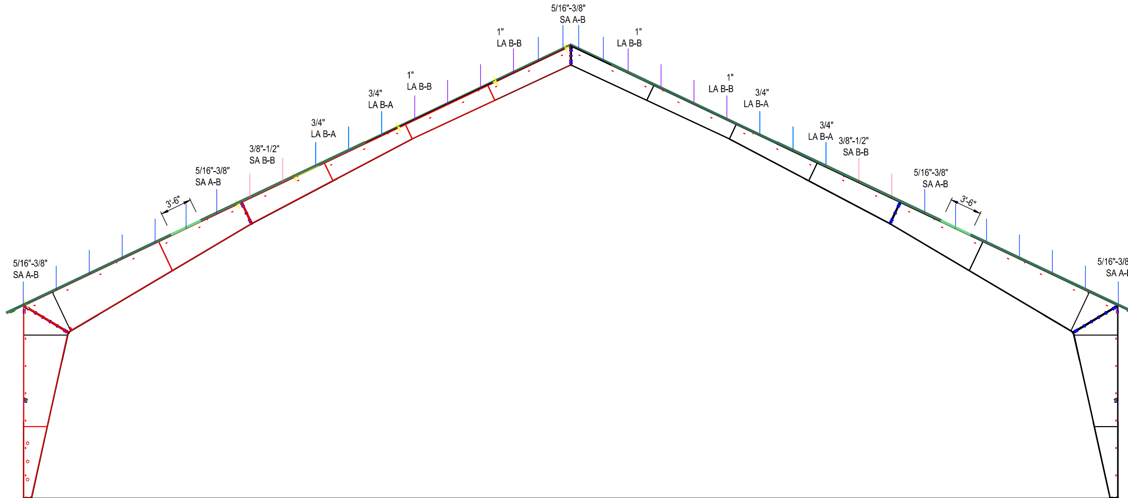
1 EXTRUSION LAYOUT COMMON FRAMES
