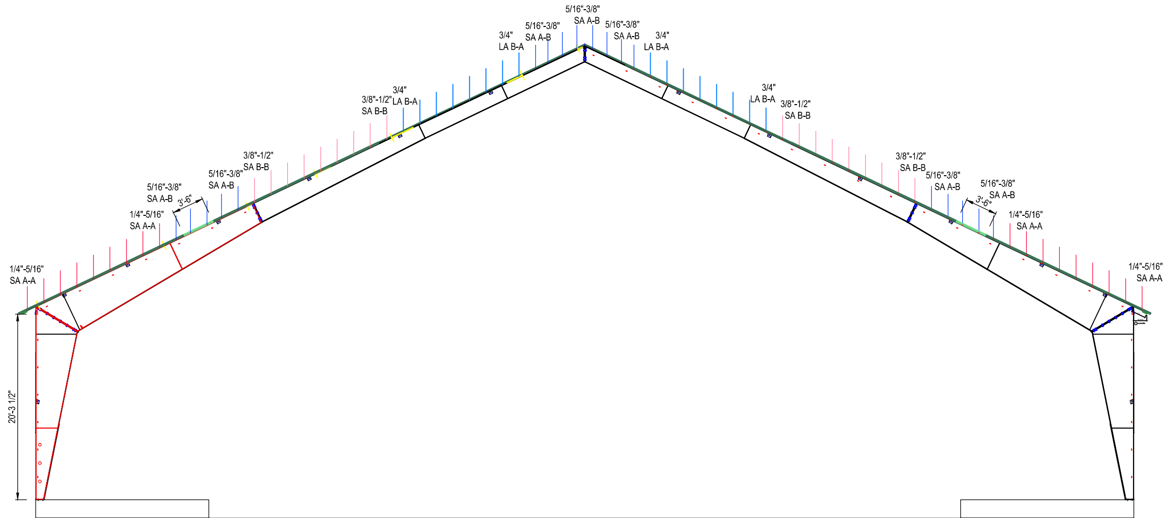
1 EXTRUSION LAYOUT FRAME LINE 1
