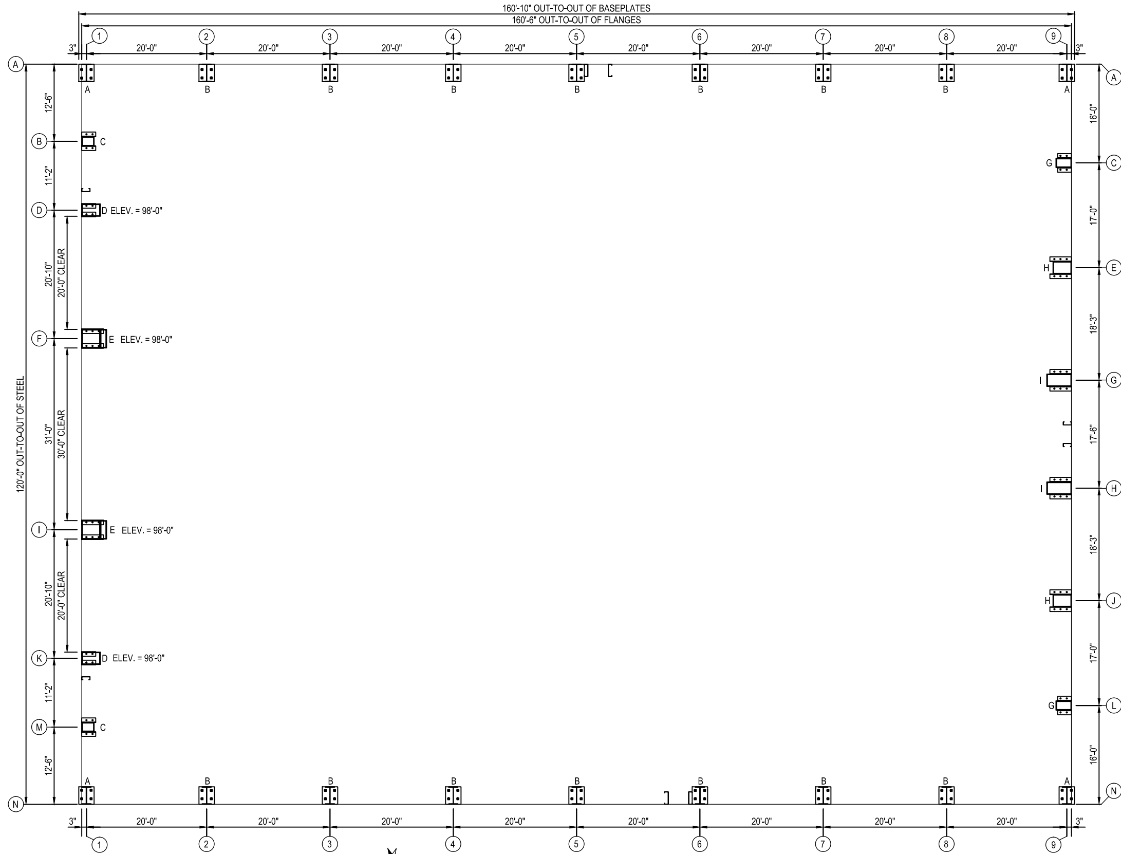
1 BASEPLATE LAYOUT ALL BASEPLATES @ ELEV. 100'-0" U.N.O.
