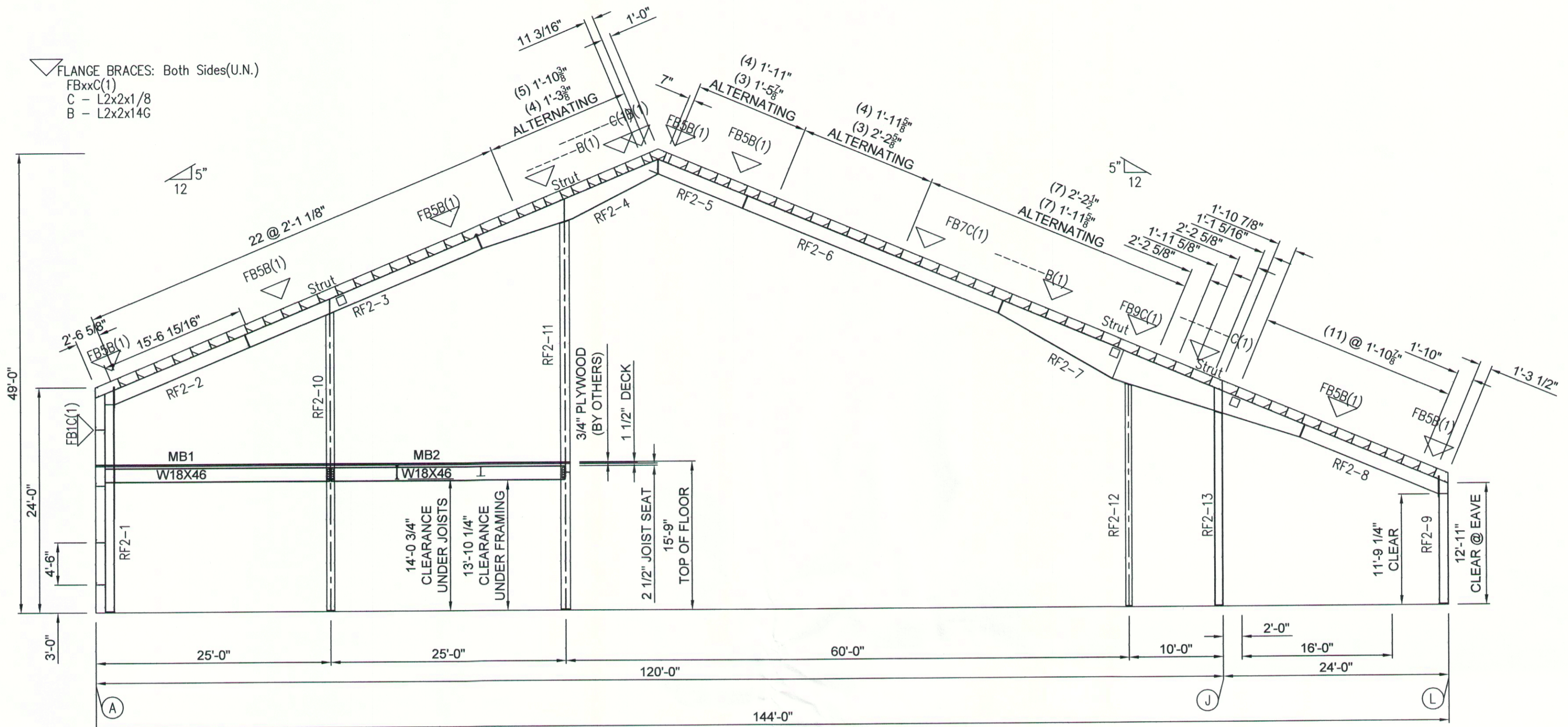
Main Frame ELEVATION: FRAME LINE 6.1
