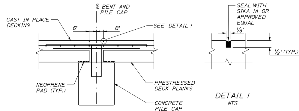
CONTROL JOINT DETAIL
