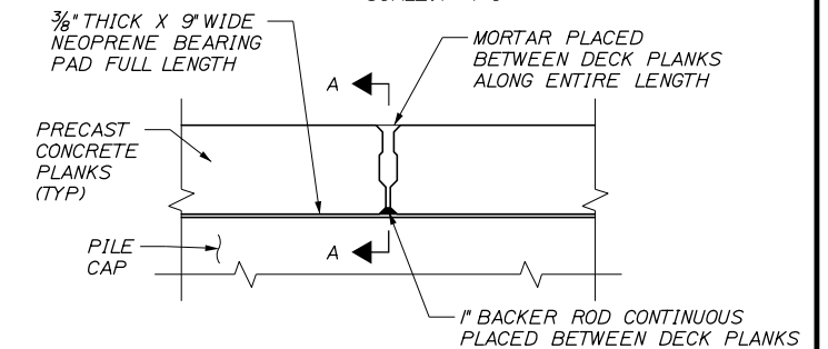
DECK PLANK ASSEMBLY DETAIL
