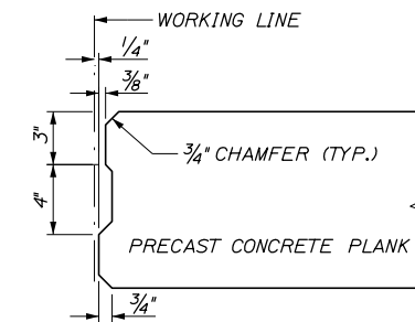
SHEAR KEY DETAIL
