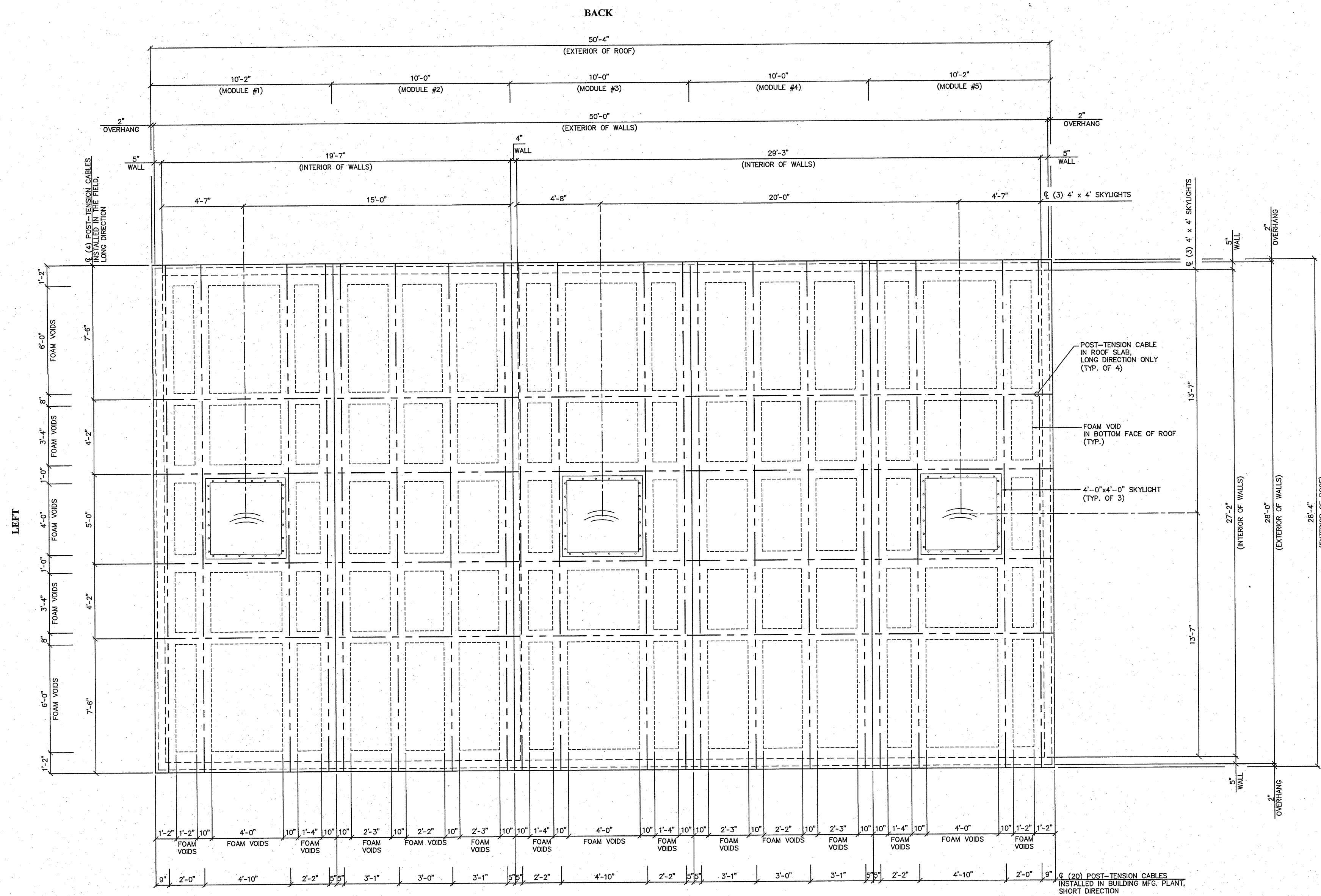
FRONT PLAN VIEW OF ROOF
