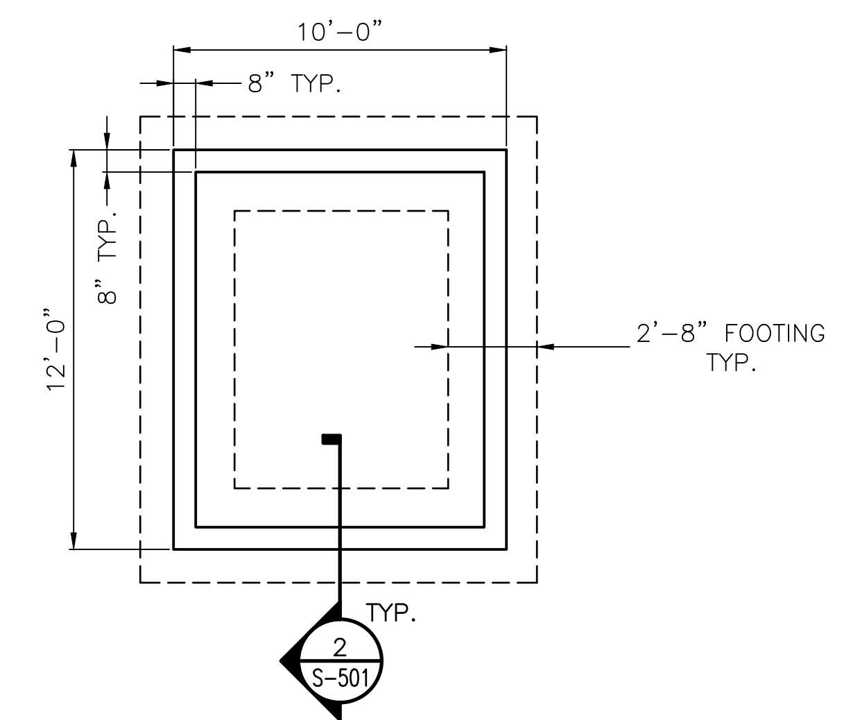
DAC BUILDING FOUNDATION PLAN
