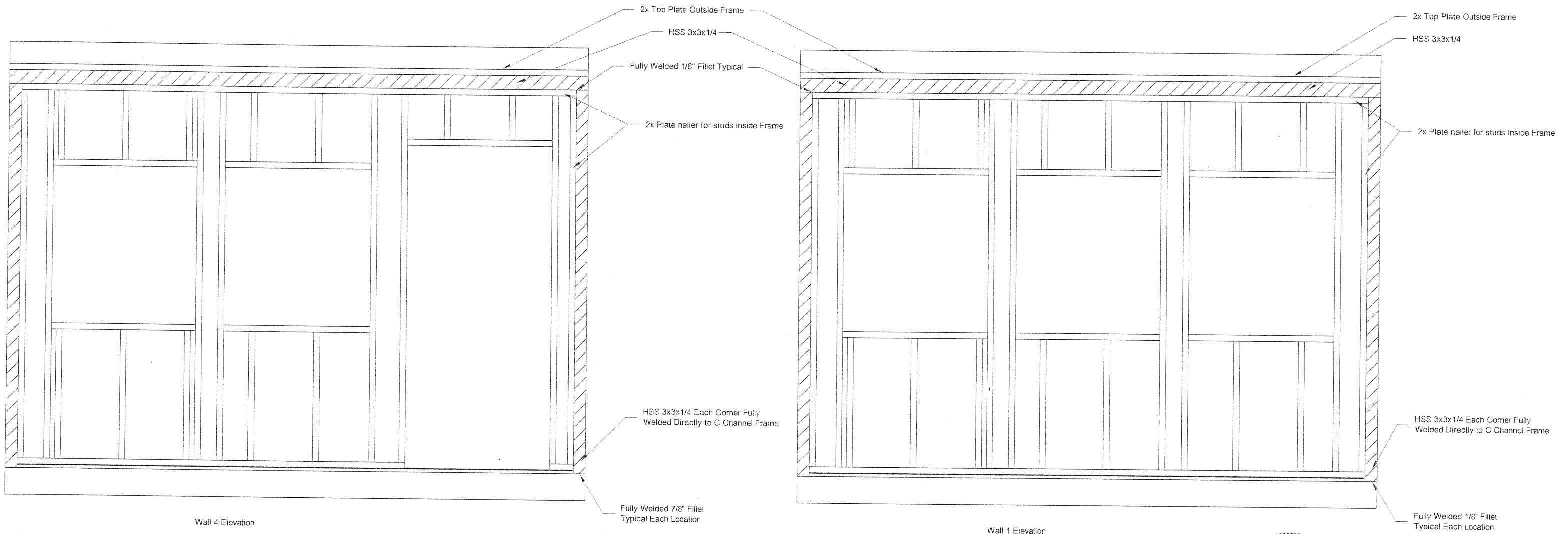
Wall 1 Elevation
