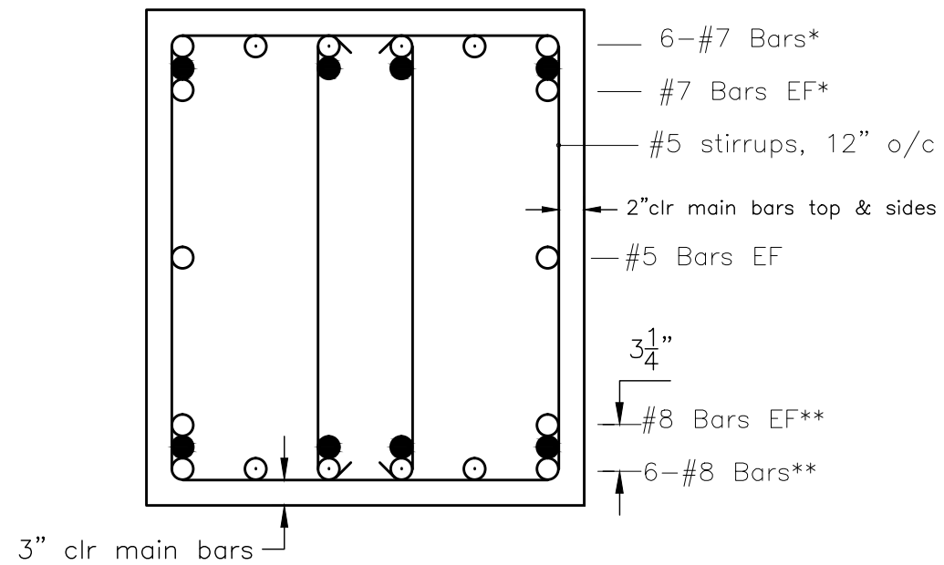
GRADE BEAM REBAR (typ UNO)
