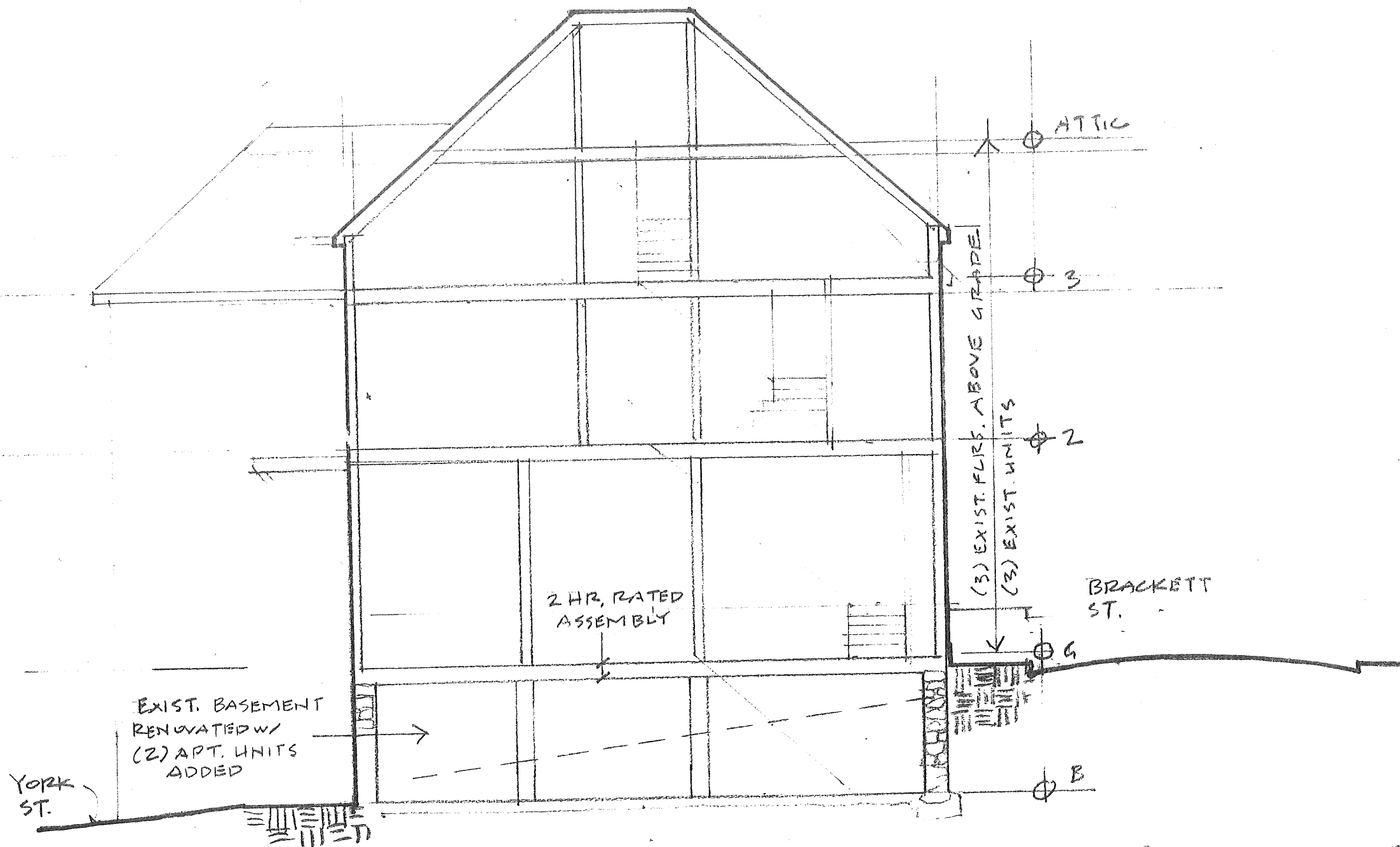
BUILDING SECTION
