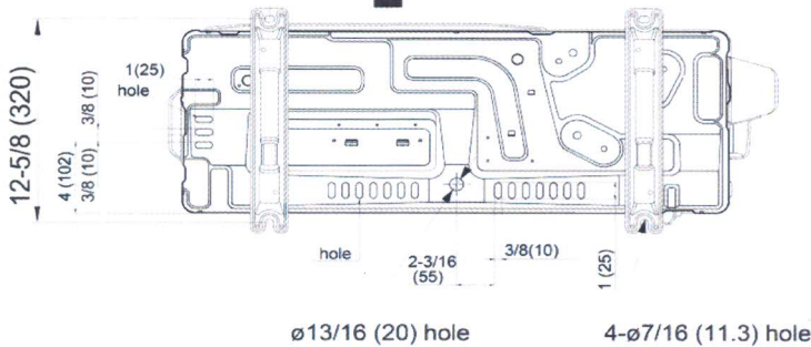
Bottom view
