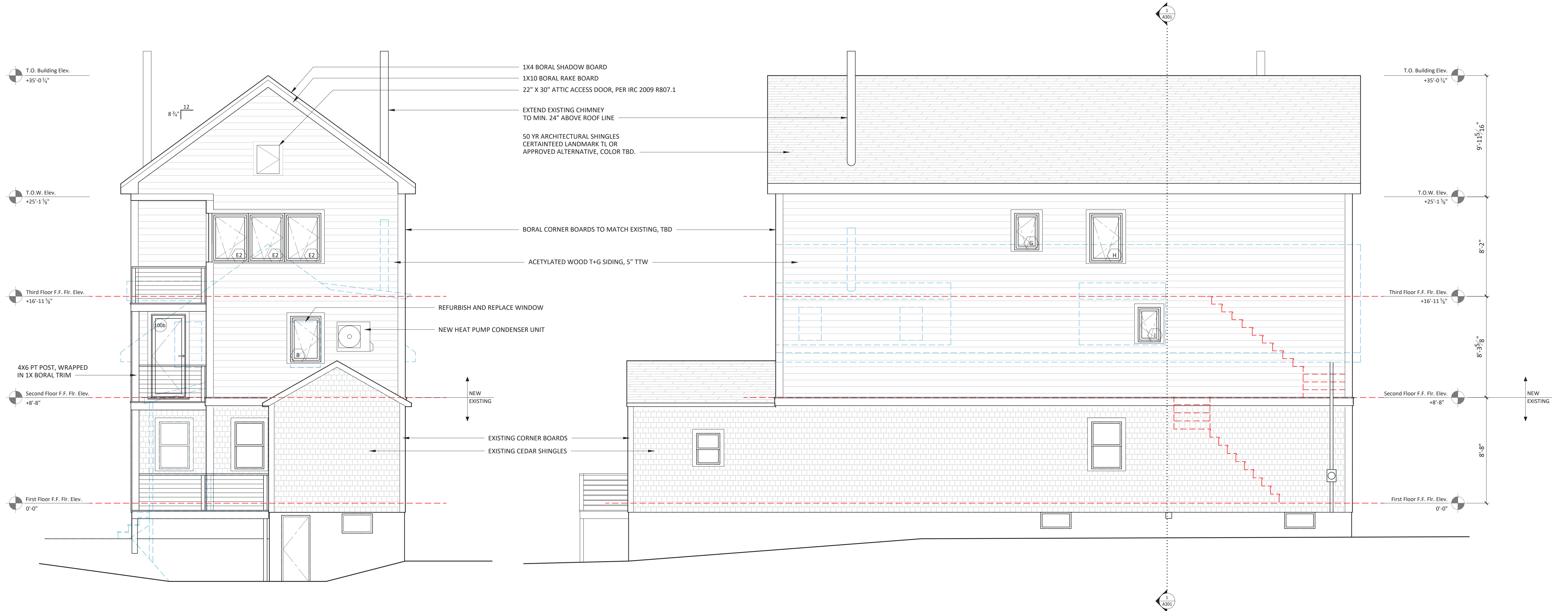
1 EAST ELEVATION \frac{1}{4}'' = 1'-0''
