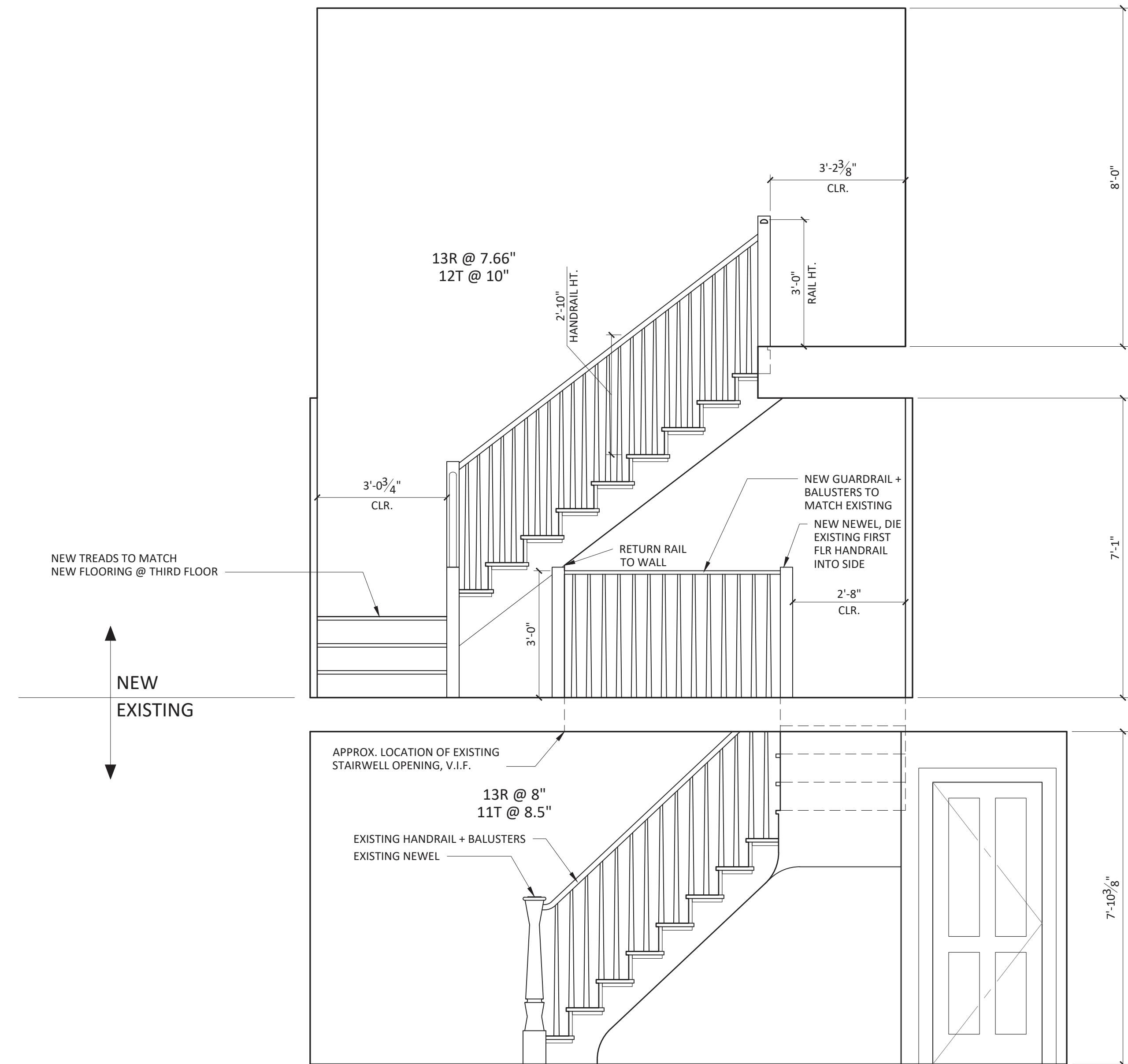
1 PRIMARY STAIRWELL - NORTH 1/2" = 1'-0"
