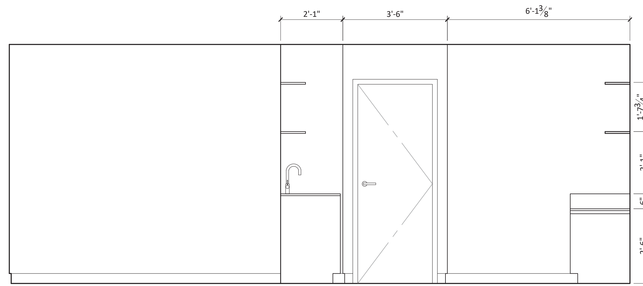
4 STUDIO - EAST 1/2" = 1'-0"
