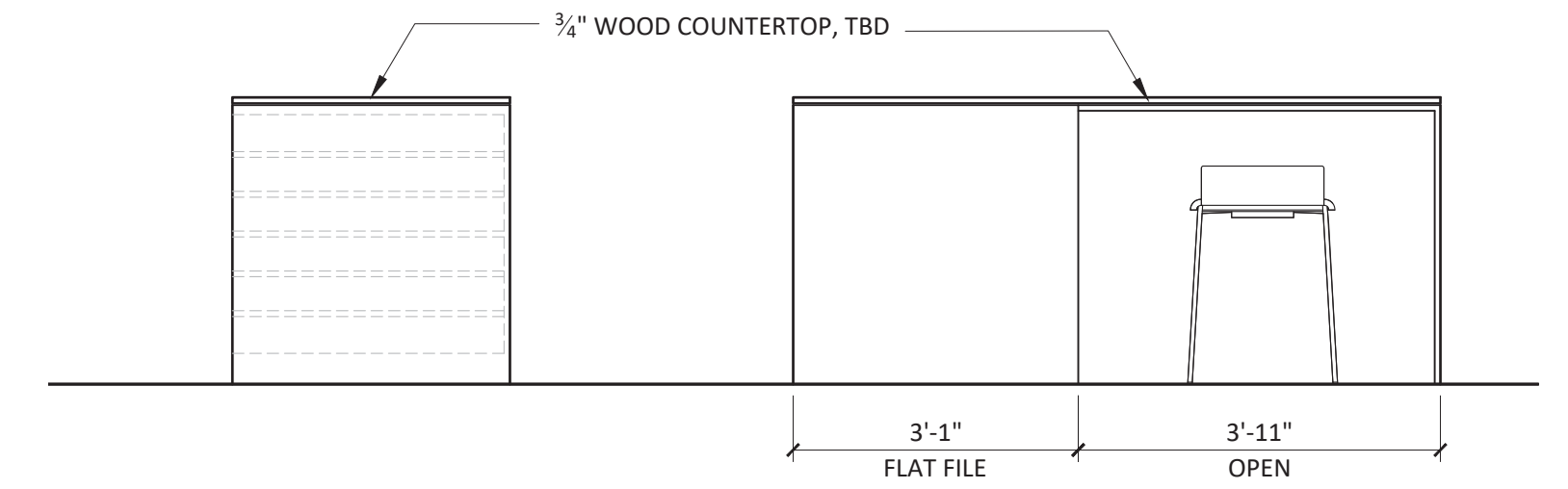
4 STUDIO - ISLAND 1/2" = 1'-0"
