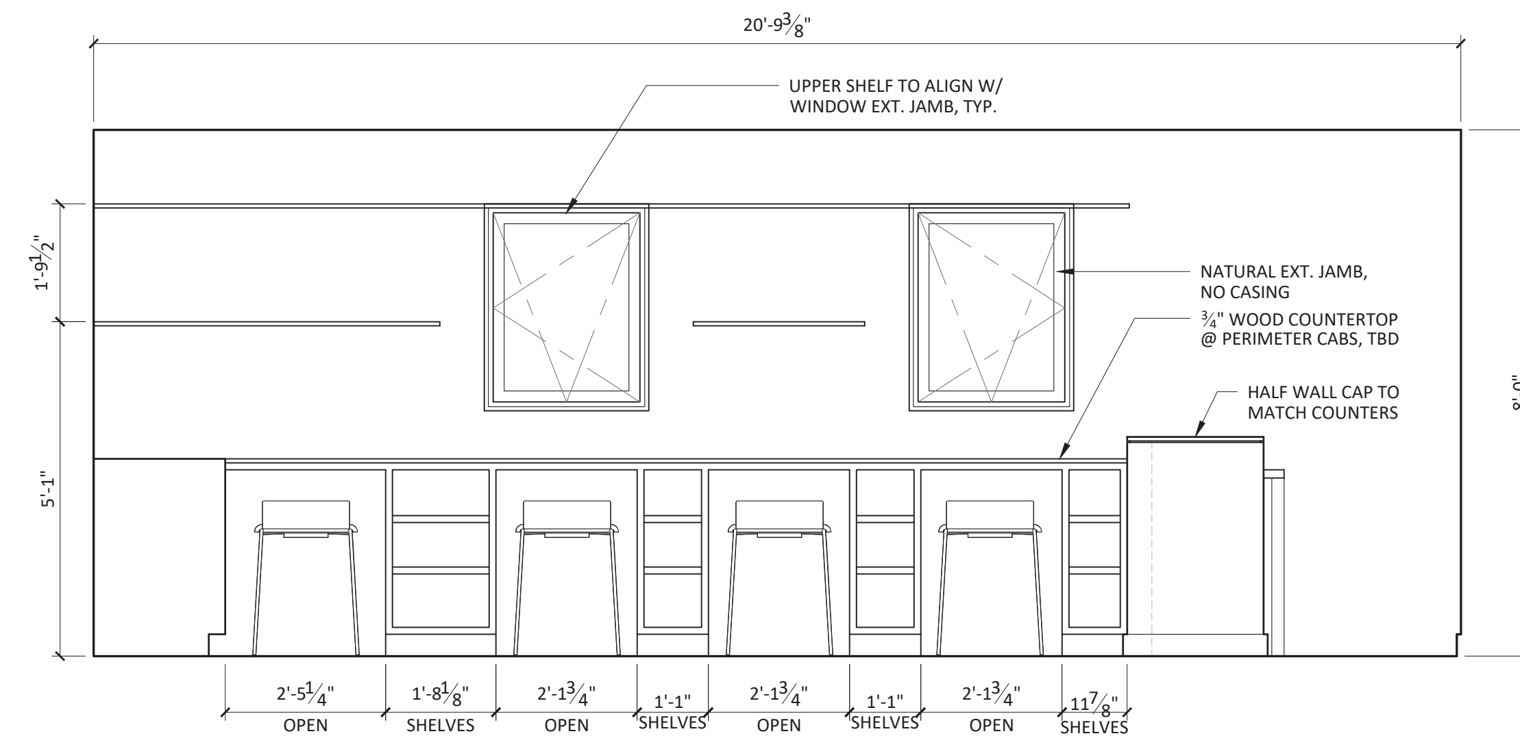
2 STUDIO - WEST 1/2" = 1'-0"
