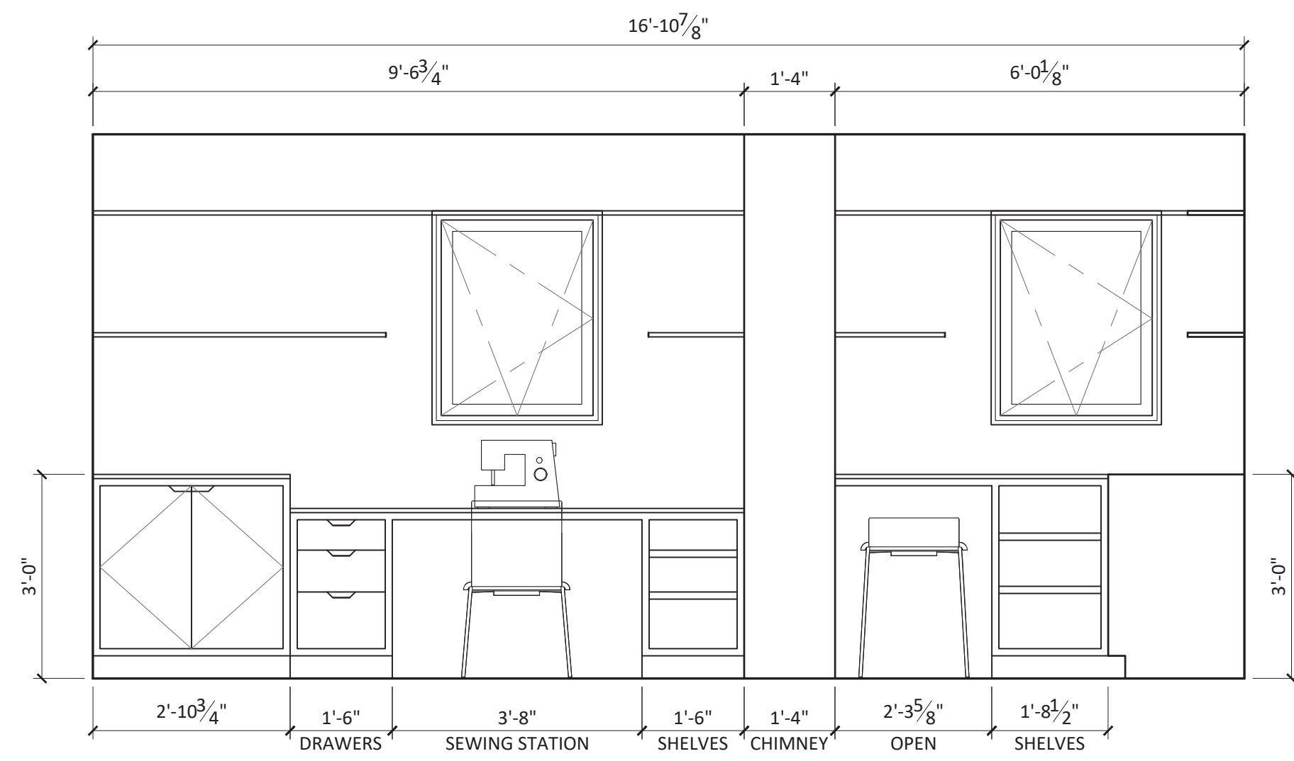
1 STUDIO - SOUTH 1/2" = 1'-0"
