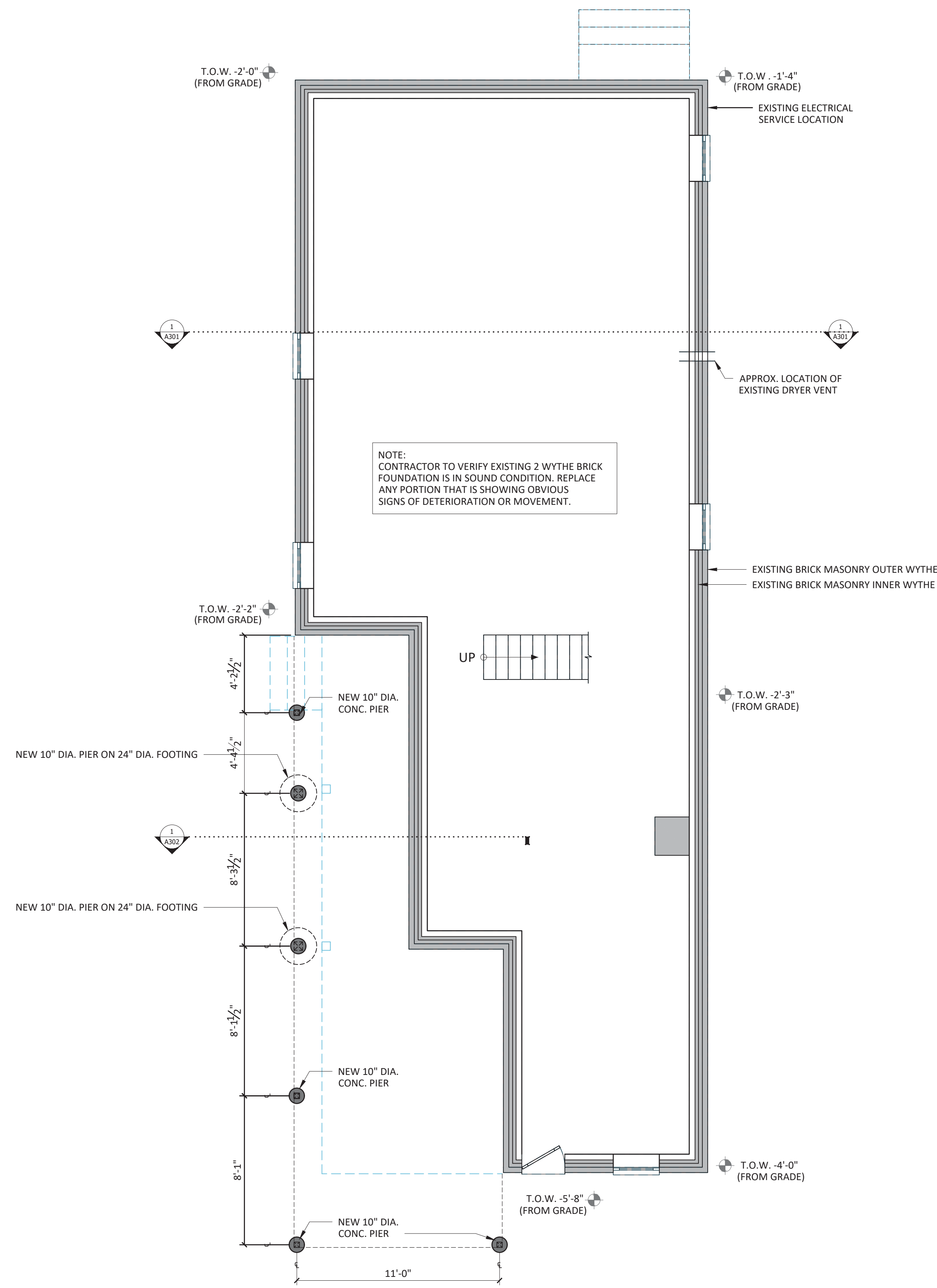
1 FOUNDATION PLAN 3/4" = 1'-0"
