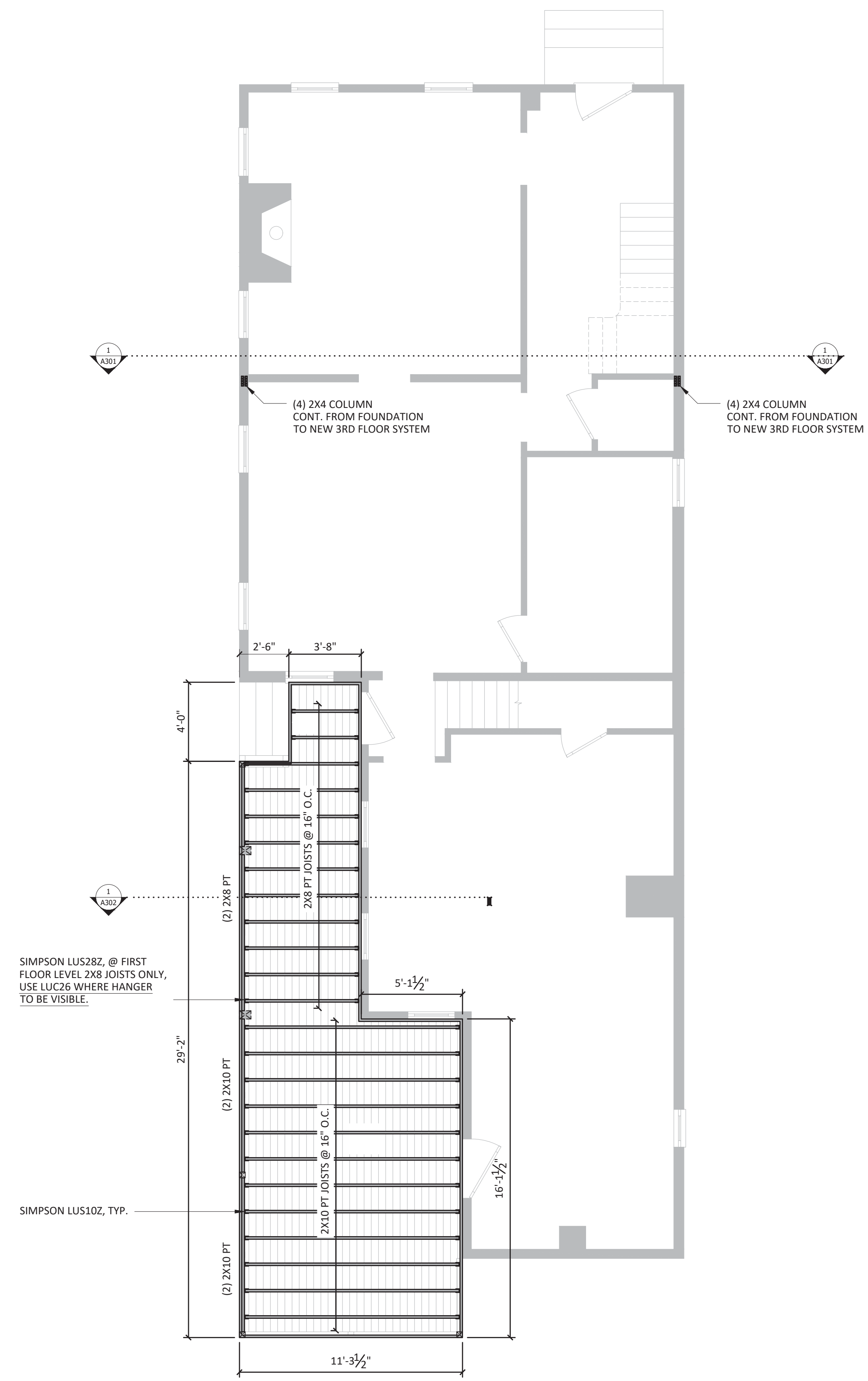
2 FIRST FLOOR DECK FRAMING PLAN 3/4" = 1'-0"
