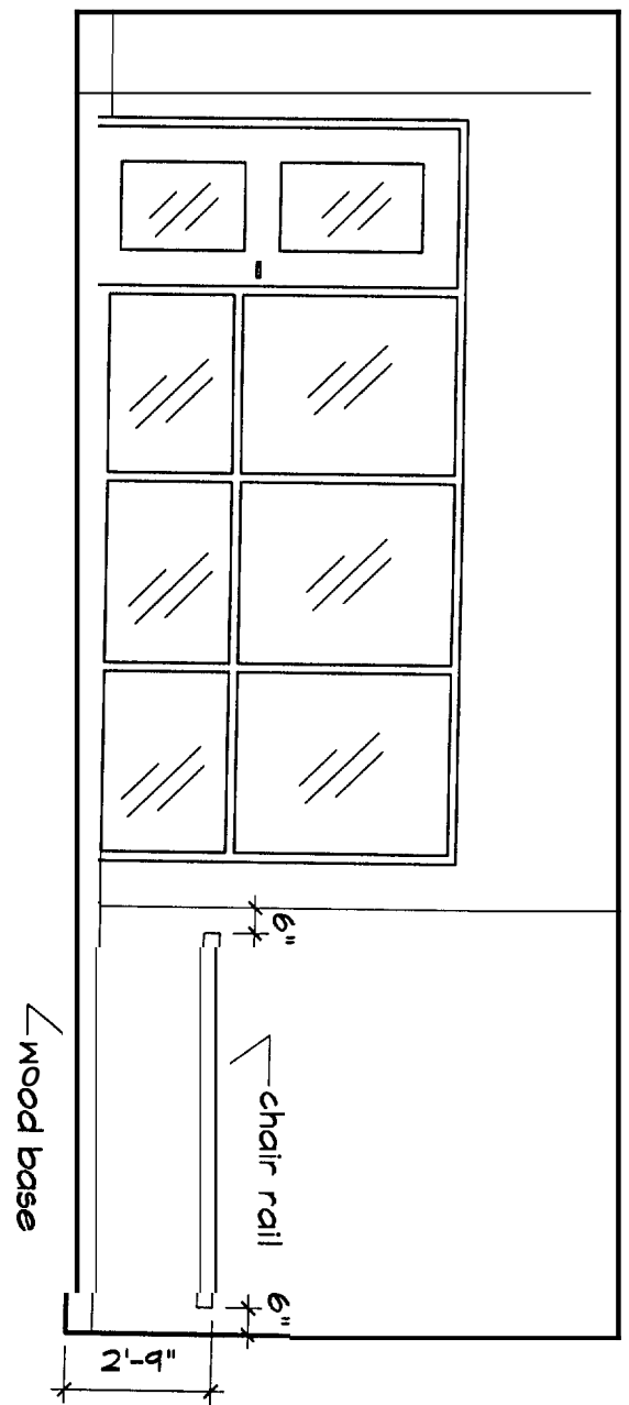
3 WAITING/CHECK-IN - WEST ELEVATION 1/4" = 1'-0"
