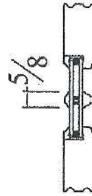
Muntin Profile
