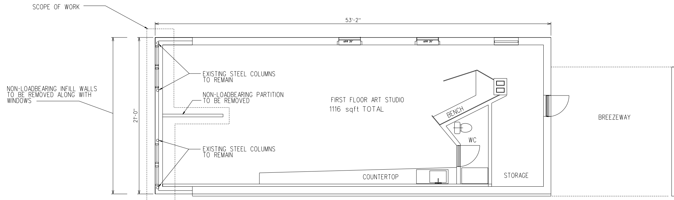
1 EXISTING FLOOR PLAN SCALE: 1/8" = 1'-0"
