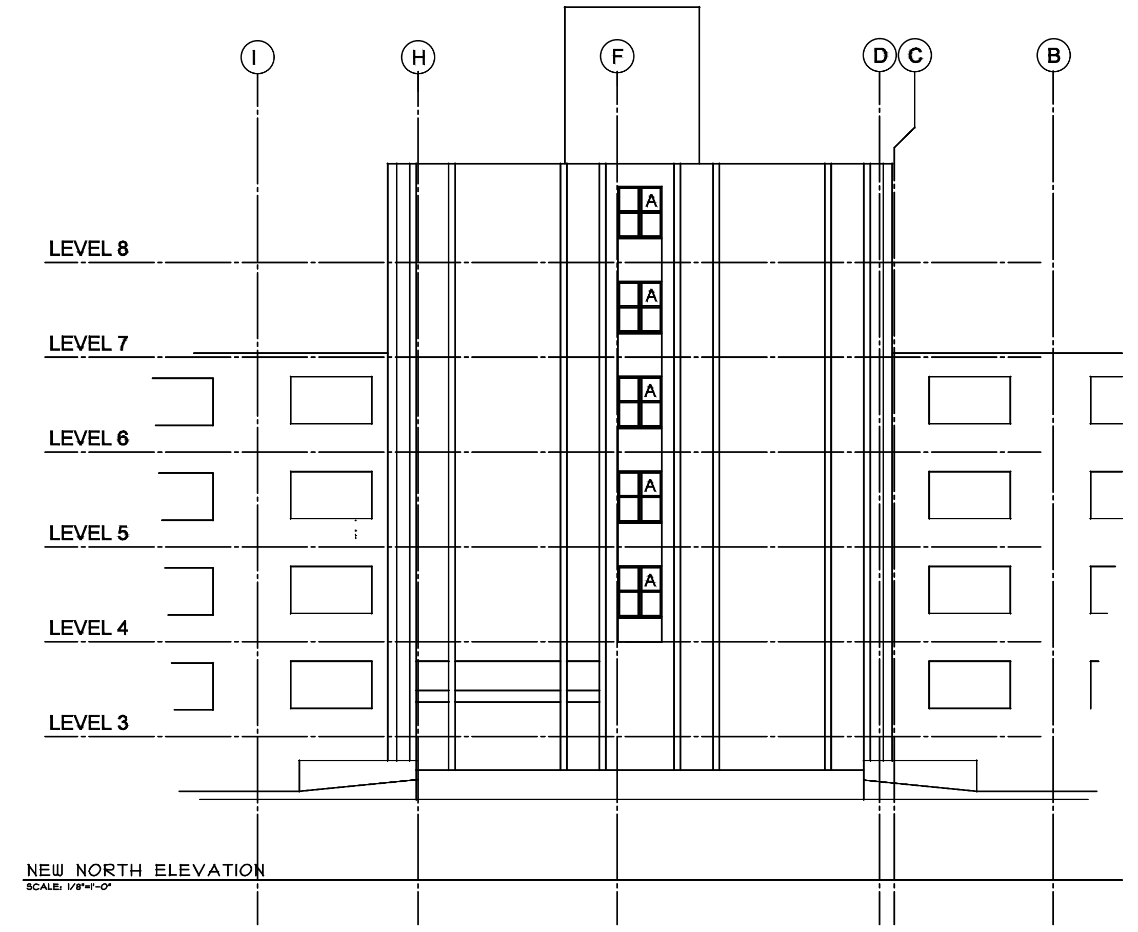
NORTH BUILDING ELEVATION ARCHITECTURAL REFERENCE: A5
