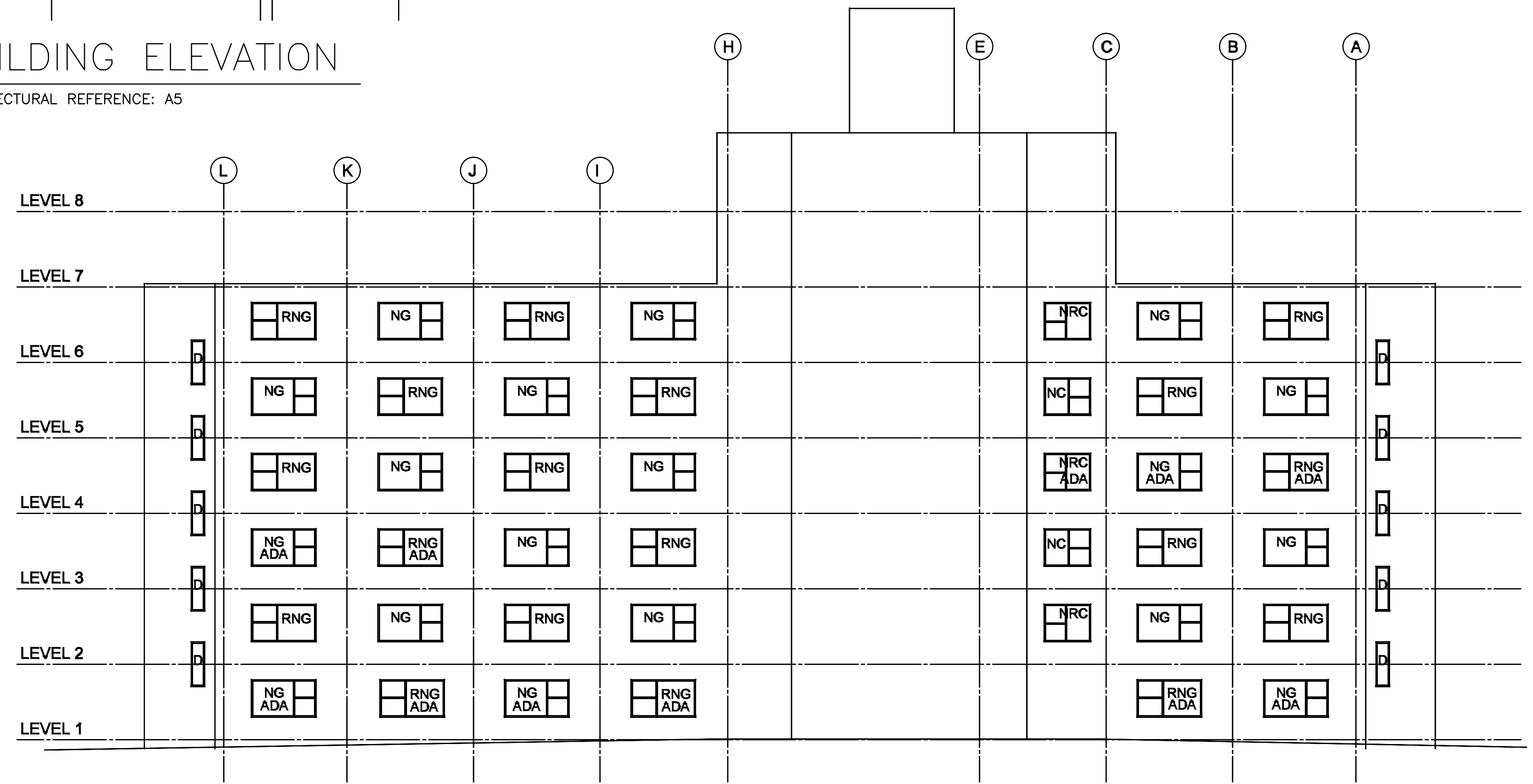
NORTH BUILDING ELEVATION ARCHITECTURAL REFERENCE: A5
