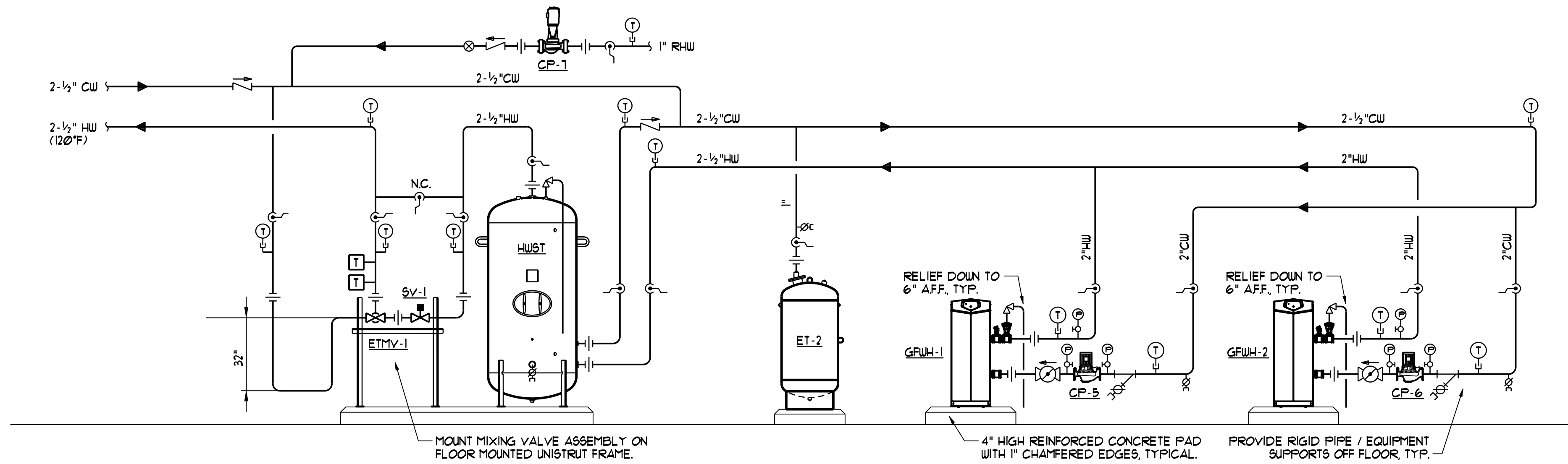
WATER HEATER PIPING SCHEMATIC
