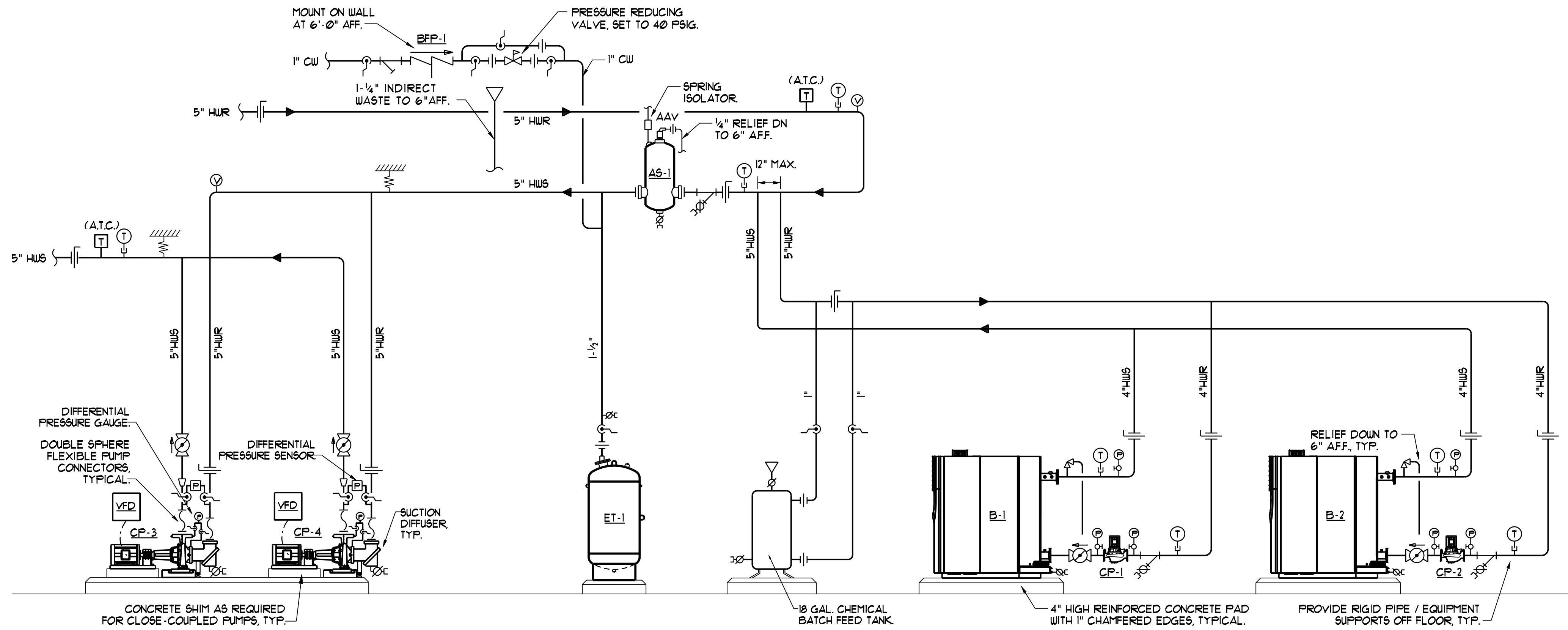
BOILER PIPING SCHEMATIC
