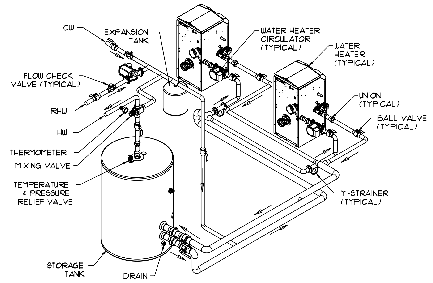
WATER HEATING ISOMETRIC
