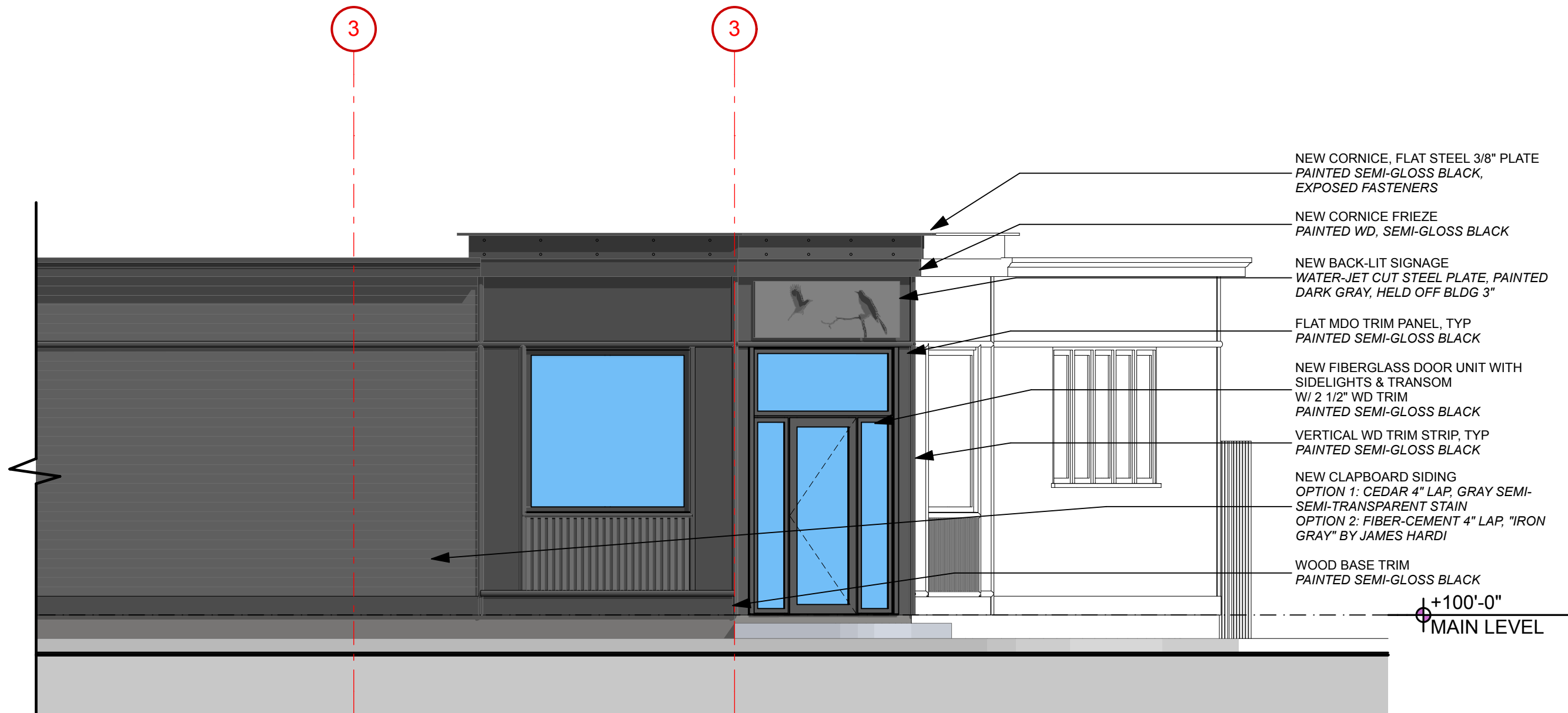
1 PARTIAL CLARK ST ELEVATION SCALE: 1/4" = 1'-0"
