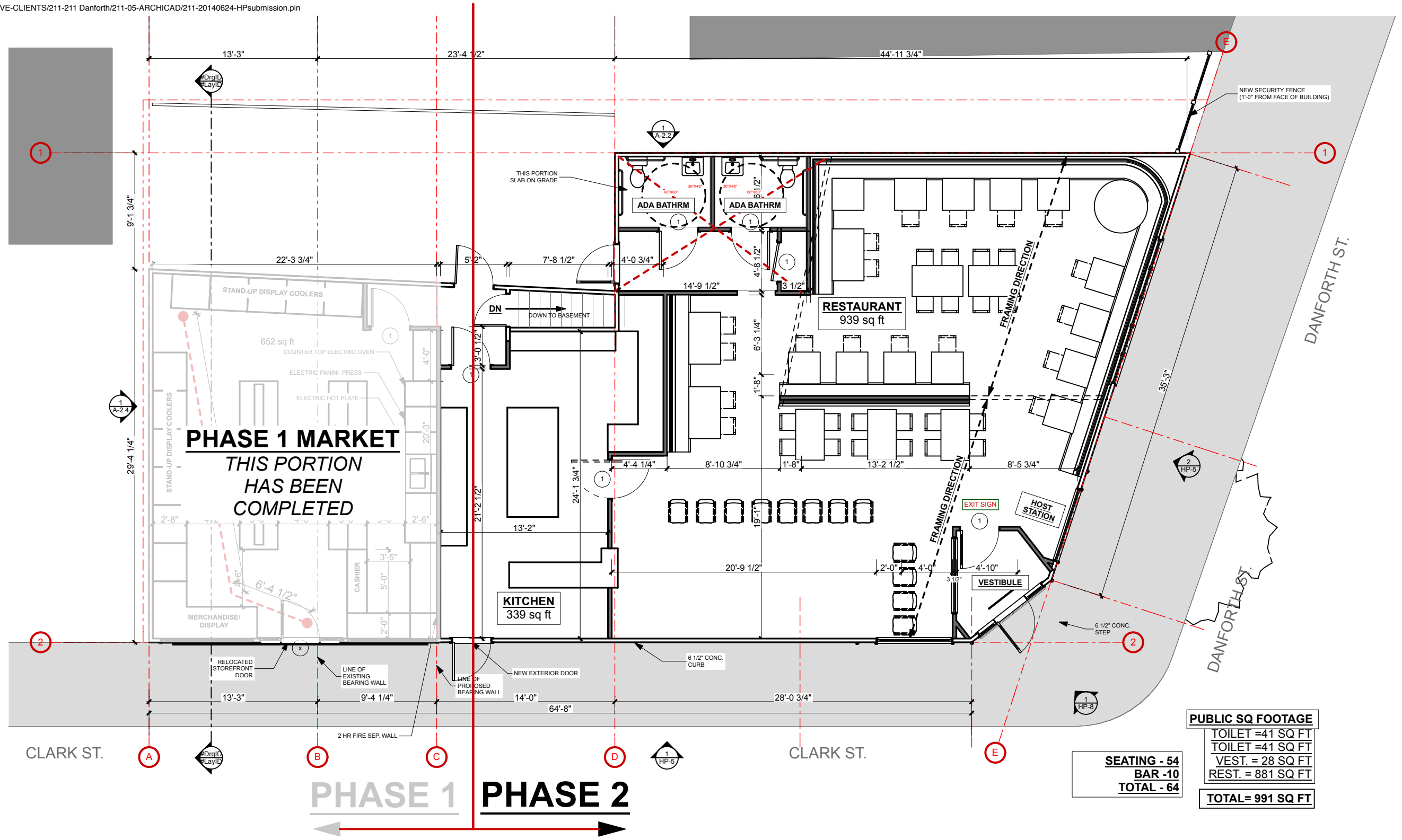
1 MAIN LEVEL FLOOR PLAN SCALE: 1/8" = 1'-0"
