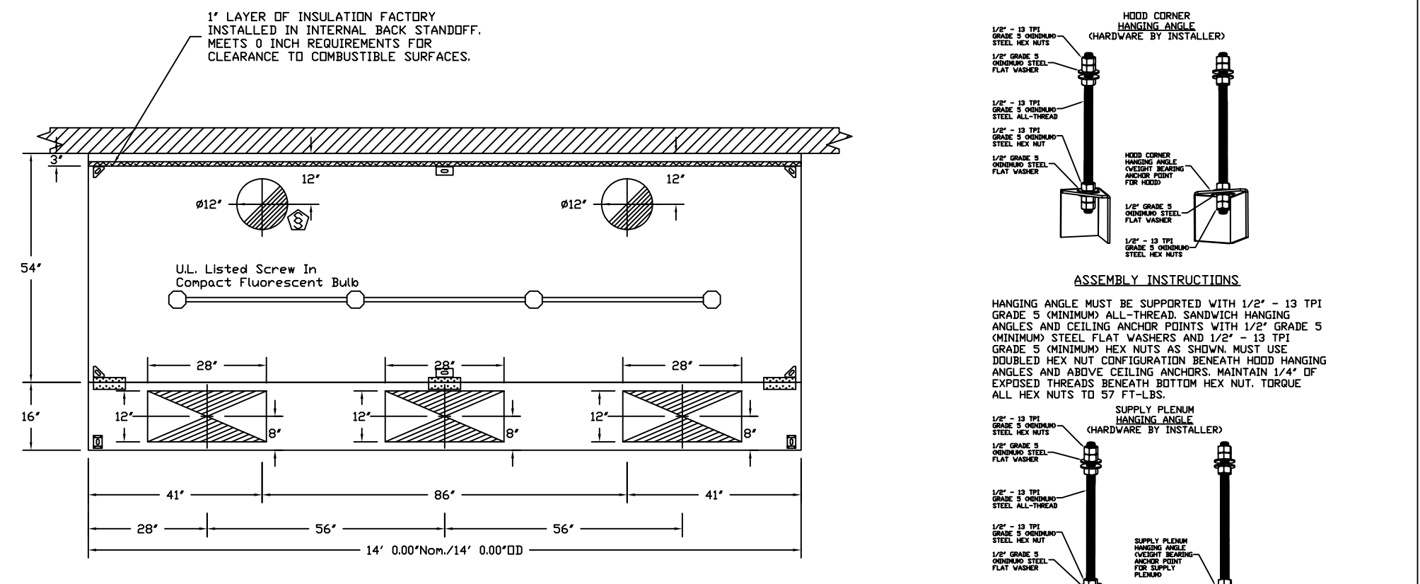
PLAN VIEW - Hood #1 14' 0.00' LONG 542ND-2-PSP-F NOTE: Additional hanging angles provided for hoods 12' and longer.
