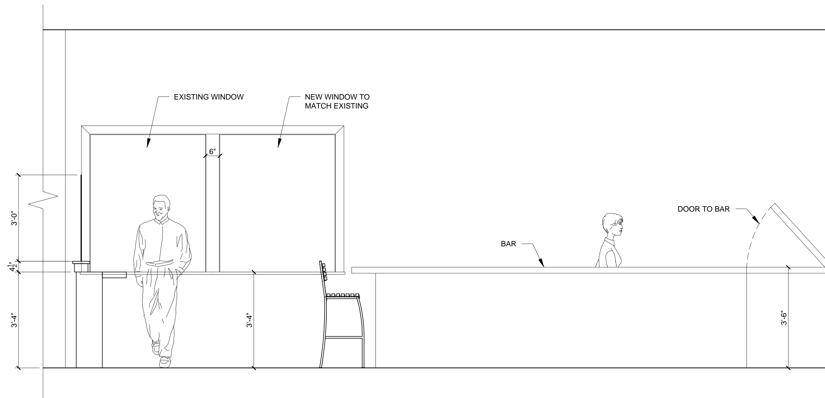
2 SECTION / ELEVATION THROUGH DINING ROOM 1 AND BAR AREA 1/2" = 1'-0"
