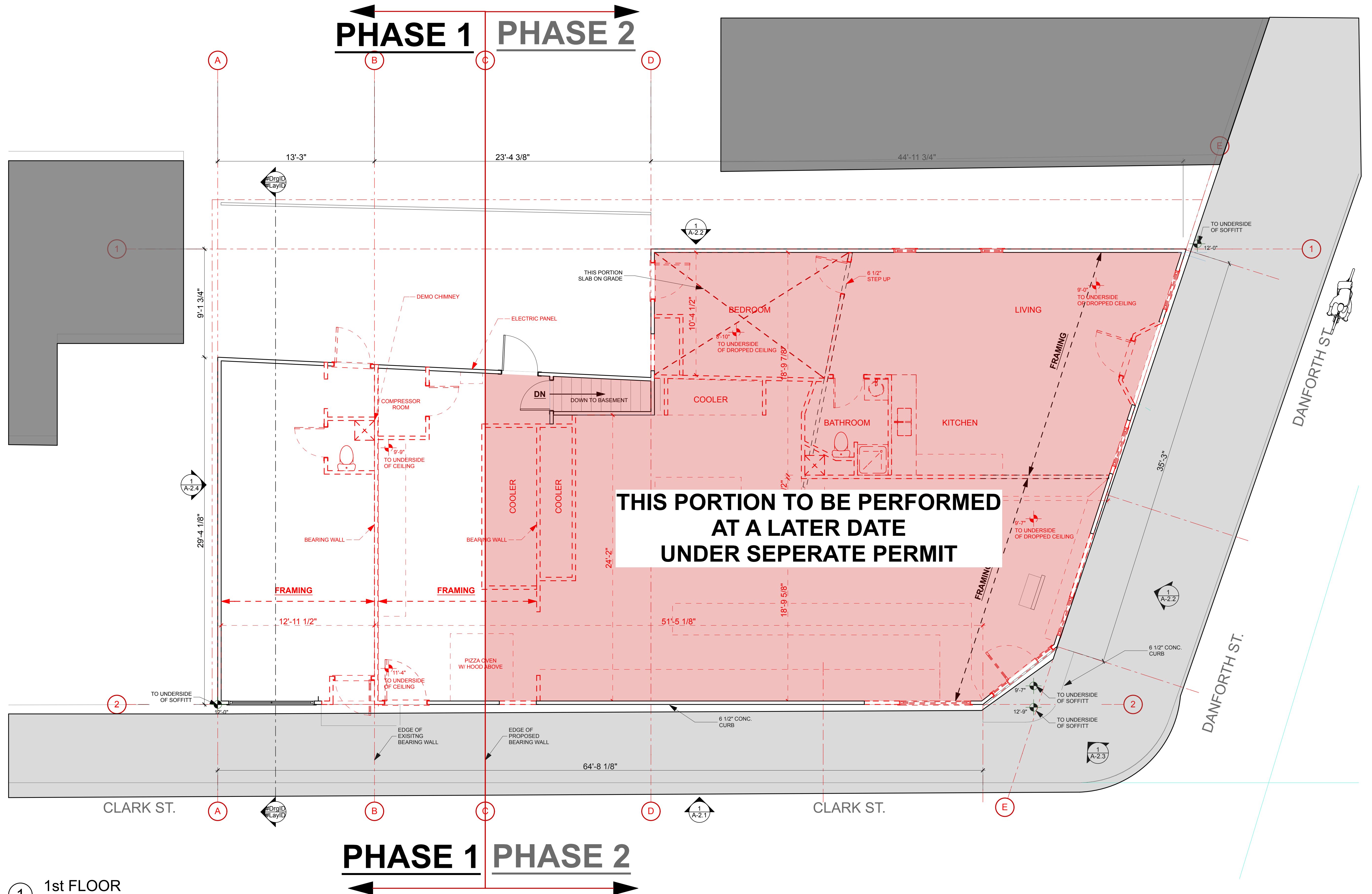
1 1st FLOOR SCALE: 1/4" = 1'-0"
