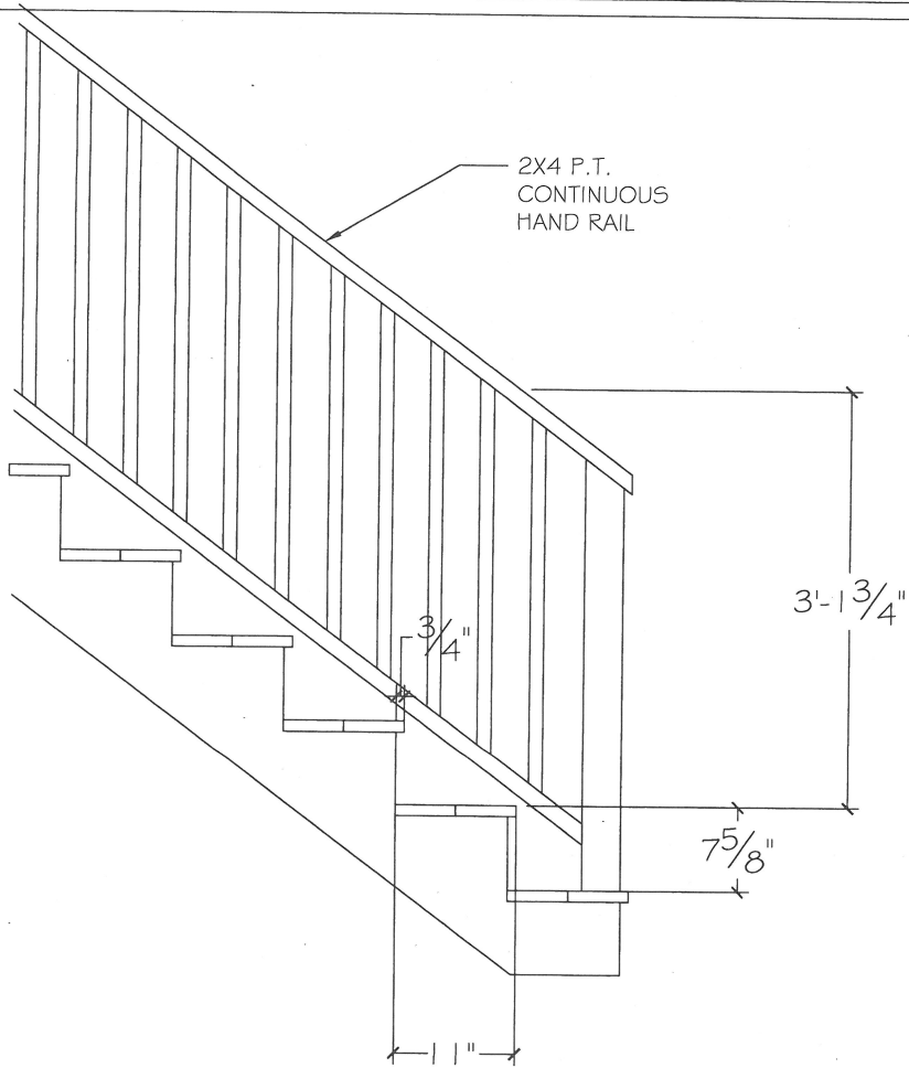
TREAD & RISER W/ RAILING DETAIL
