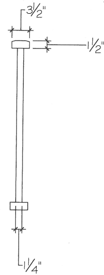
BALUSTER DETAIL
