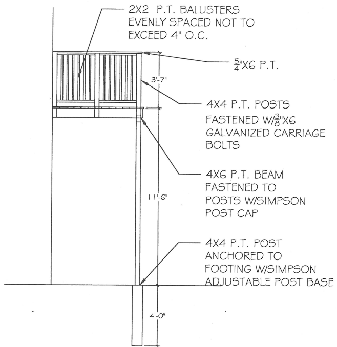
LEFT ELEVATION
