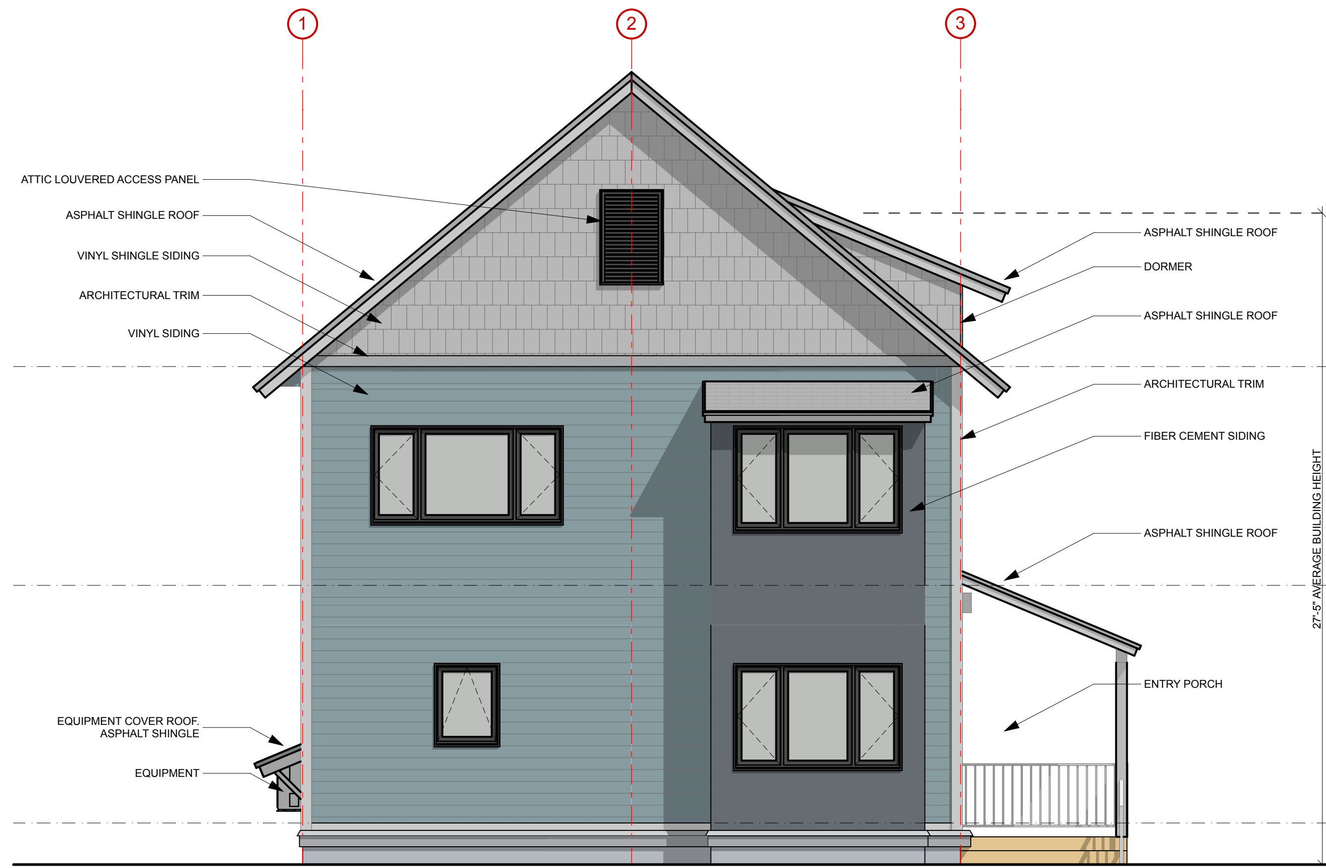
4 SW ELEVATION: MAY ST SCALE: 1/4" = 1'-0"
