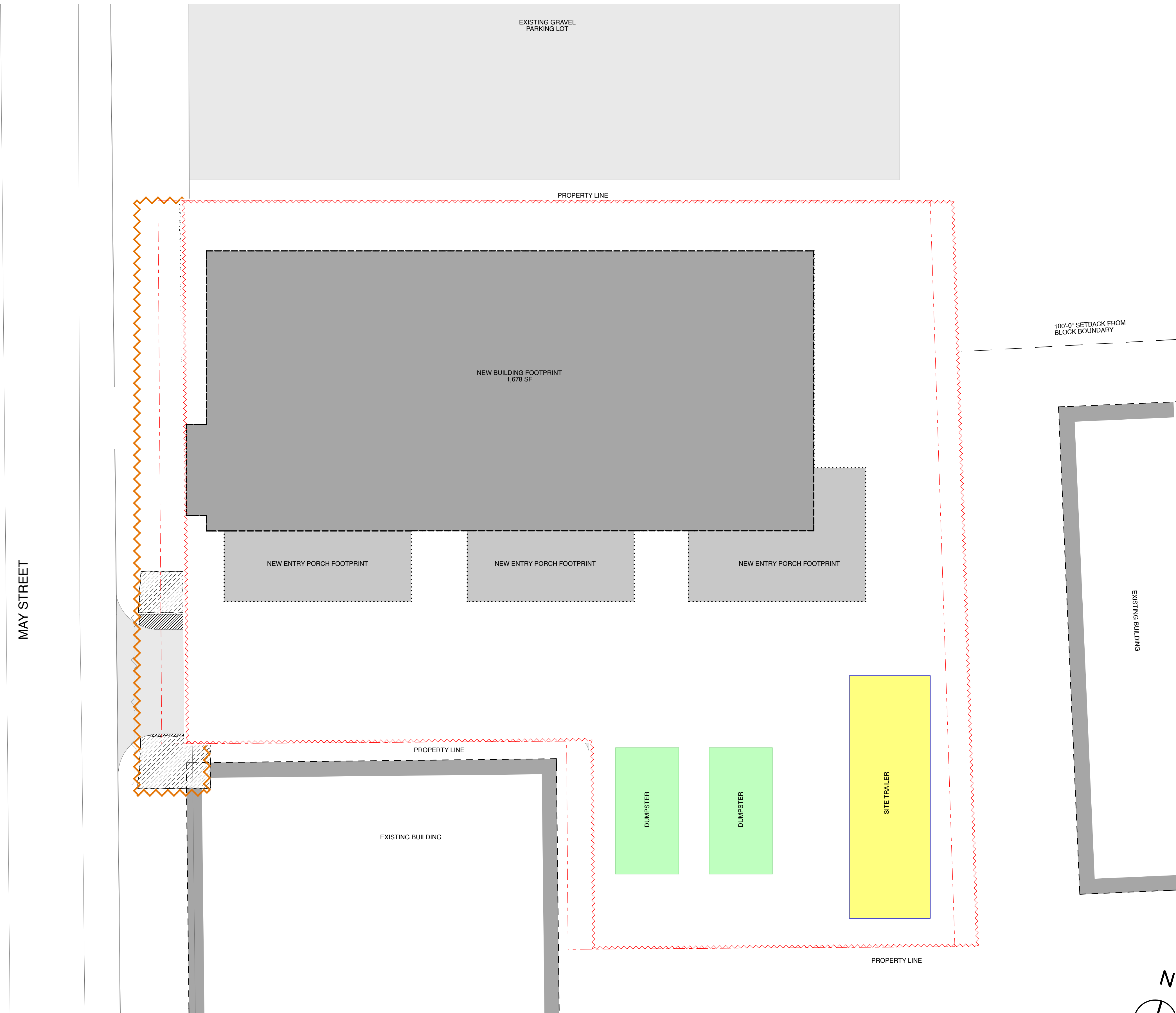
1 CONSTRUCTION MANAGEMENT PLAN SCALE: 3/16" = 1'-0"
