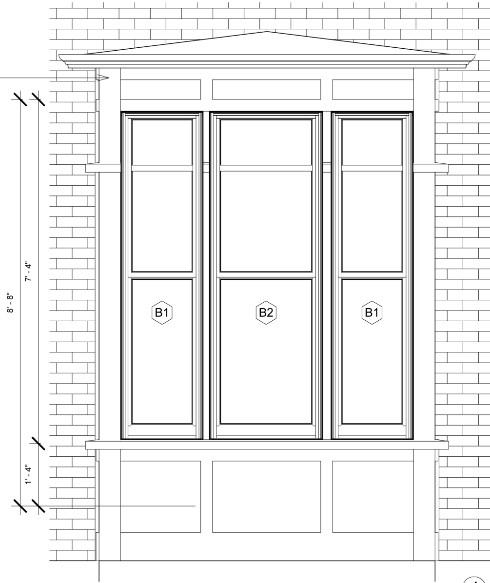
2 Bay Window - Front 1/2" = 1'-0"
