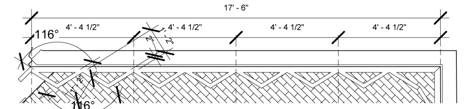
7 Varge Board Detail 1/4" = 1'-0"
