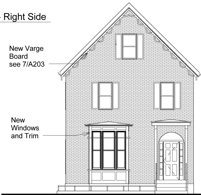
5 116 Clark Street Elevation 1" = 10'-0"
