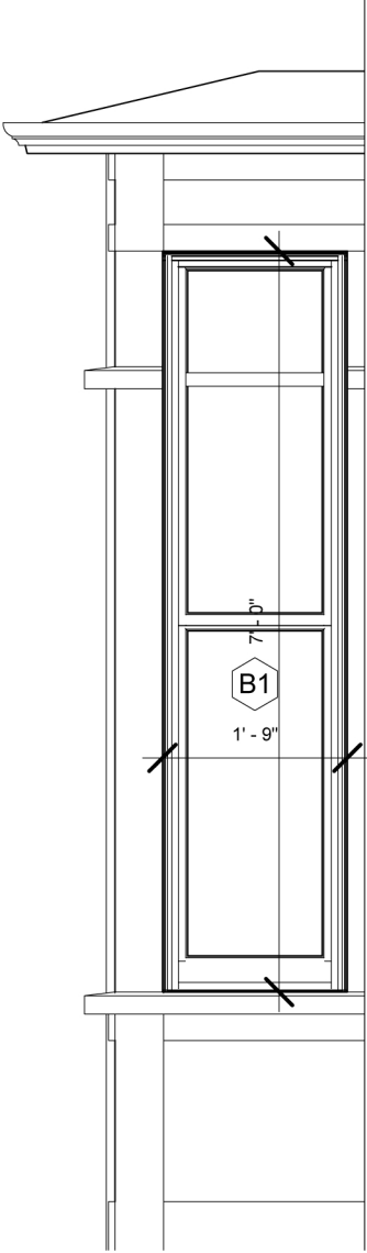
3 Bay Window - Left Side 1/2" = 1'-0"
