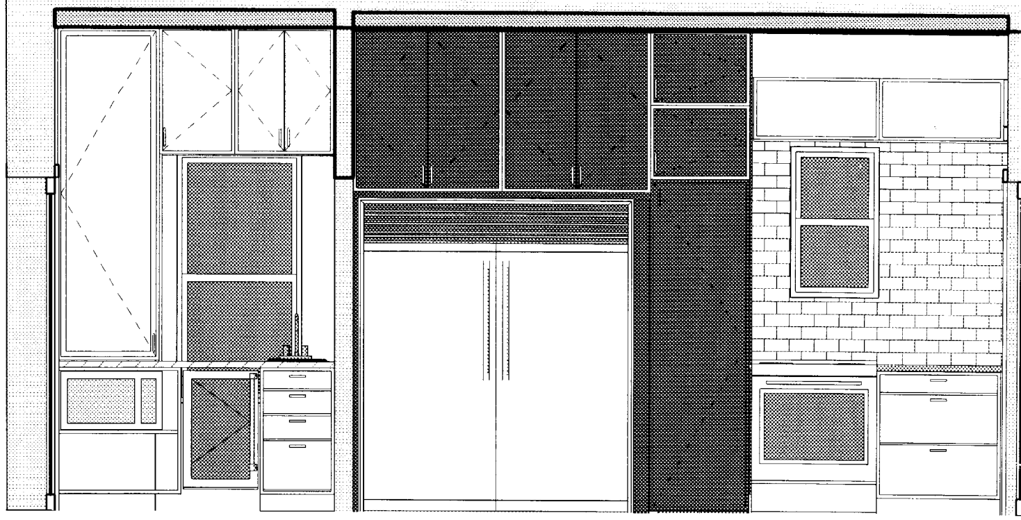
1 KIT - Main Line 3/8" = 1'-0"
