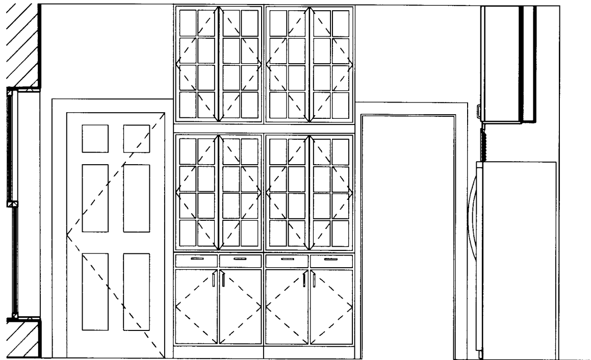
2 KIT - Cabs-Pantry 3/8" = 1'-0"
