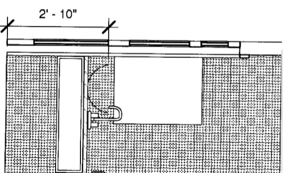
4 Bathroom - 1st - Vessel Sink 3/8" = 1'-0"
