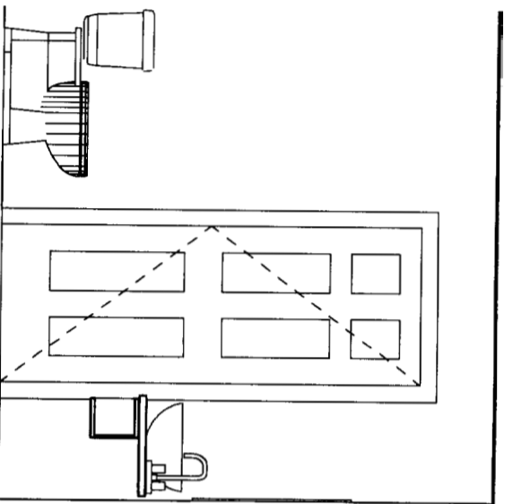
2 Bathroom - 1st - D 3/8" = 1'-0"
