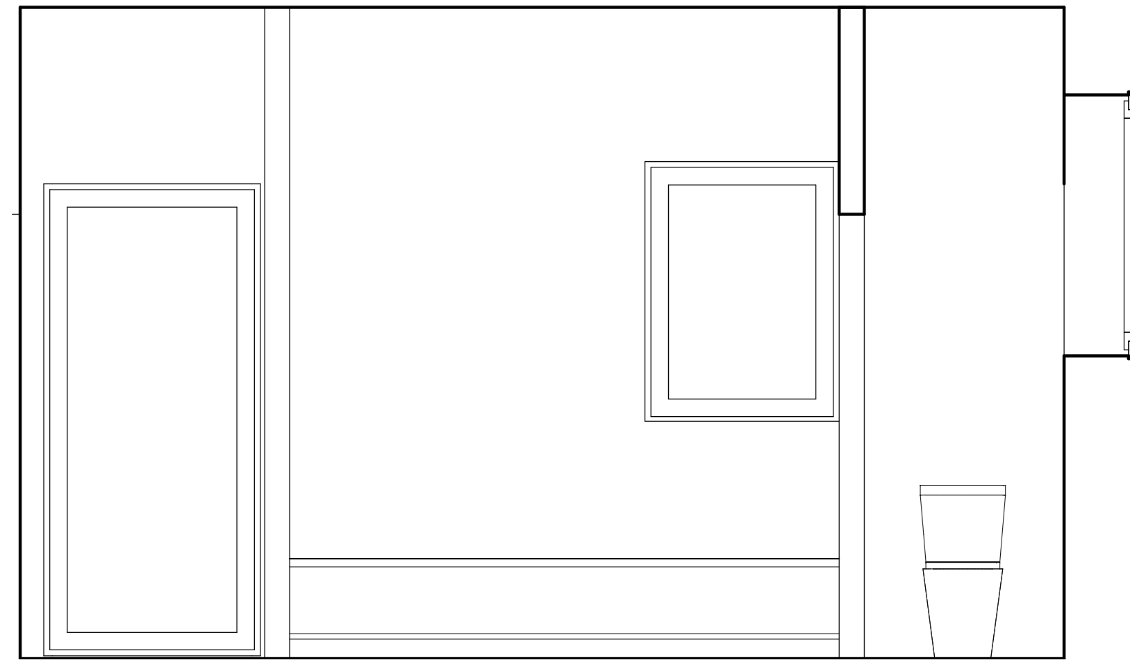
6 MUDROOM NORTH 1/2" = 1'-0"
