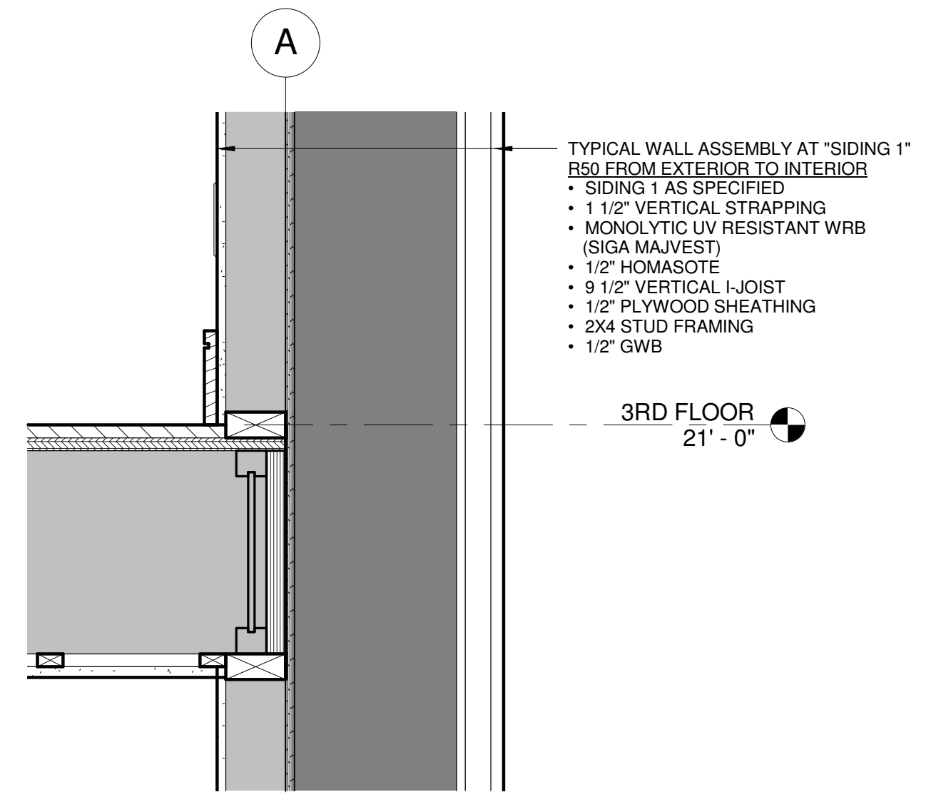
3 DETAIL - EDGE OF FLOOR 1 1/2" = 1'-0"
