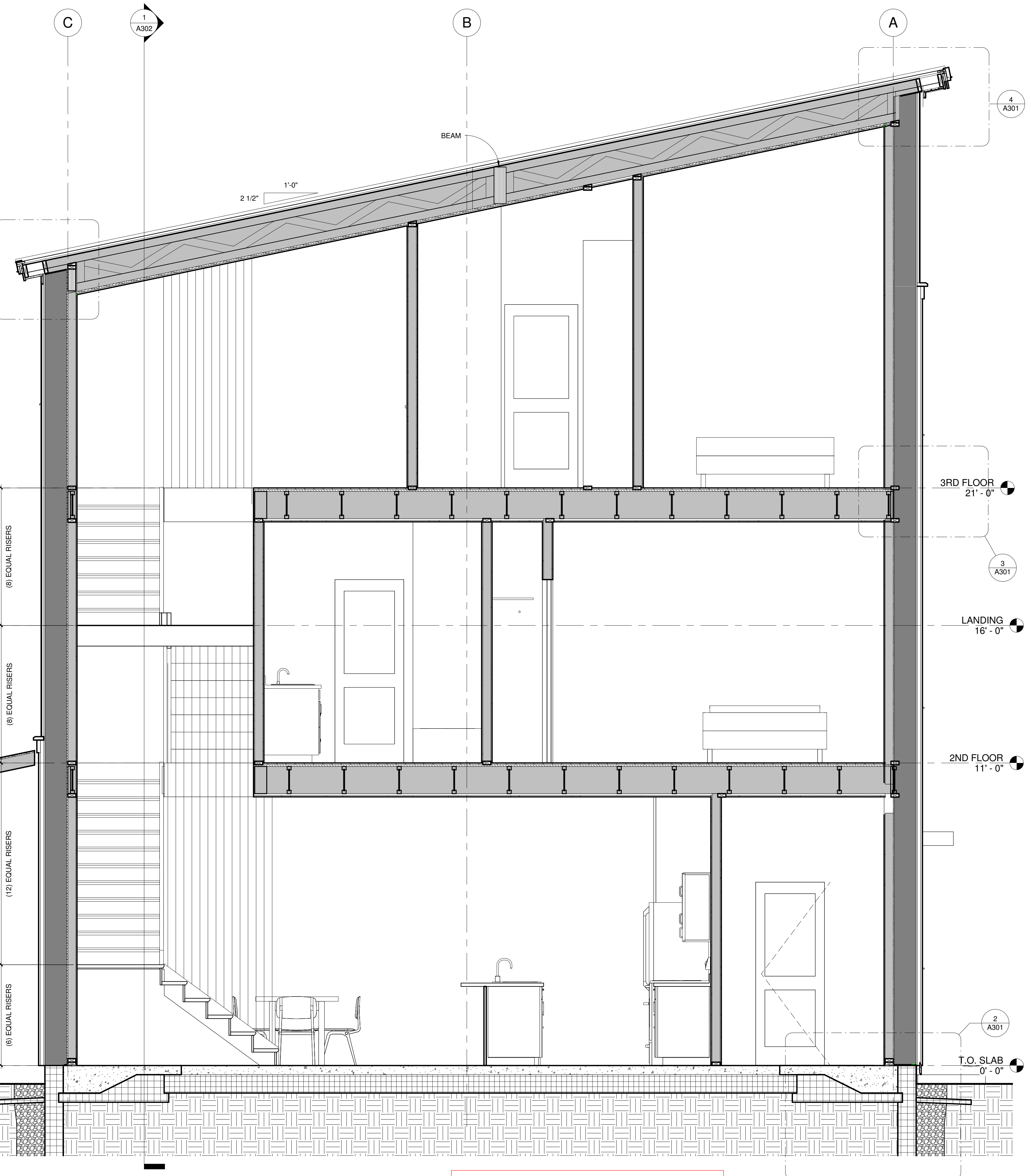
1 BUILDING SECTION 1 1/2" = 1'-0"
