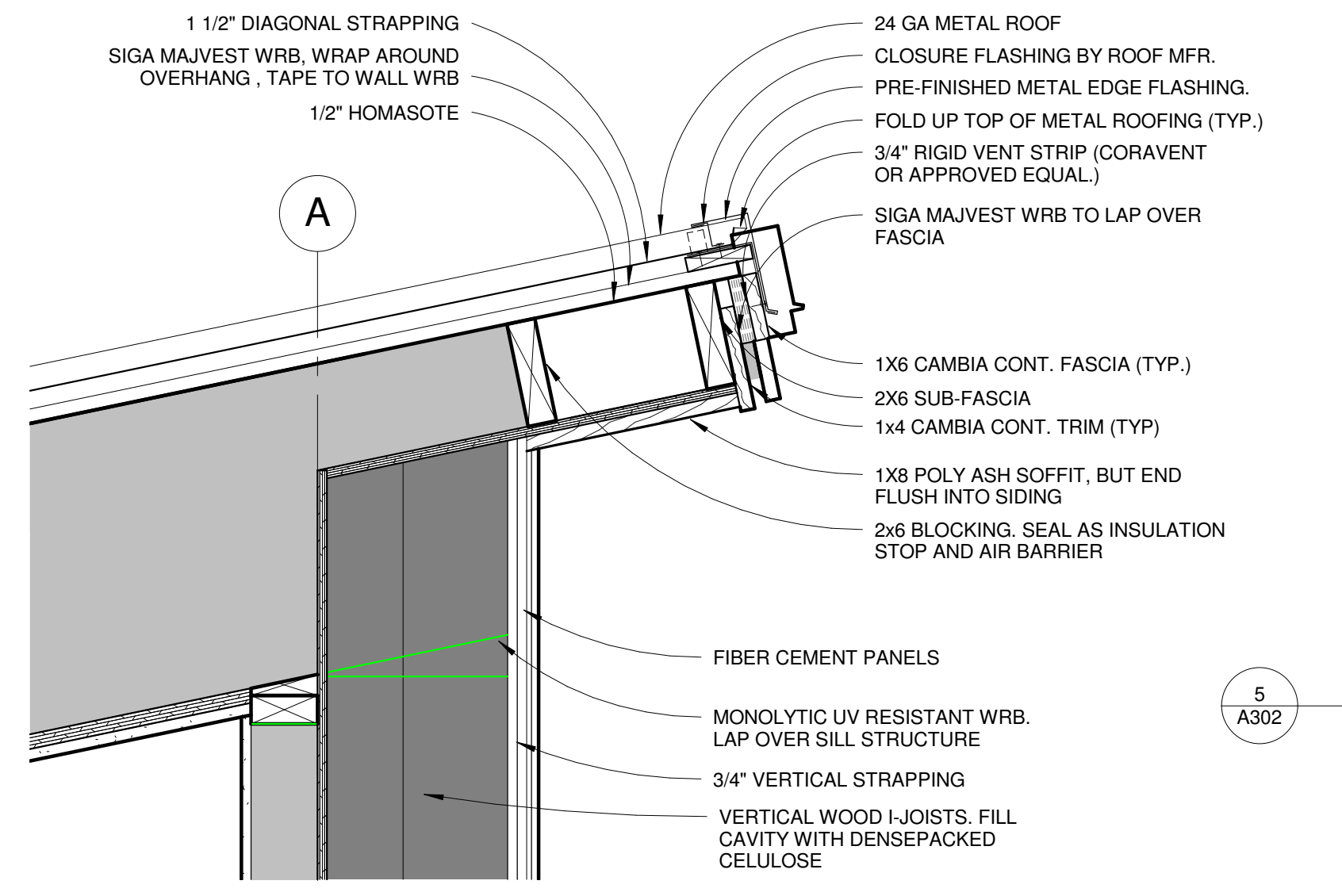
4 DETAIL - HIGH EAVE 1 1/2" = 1'-0"
