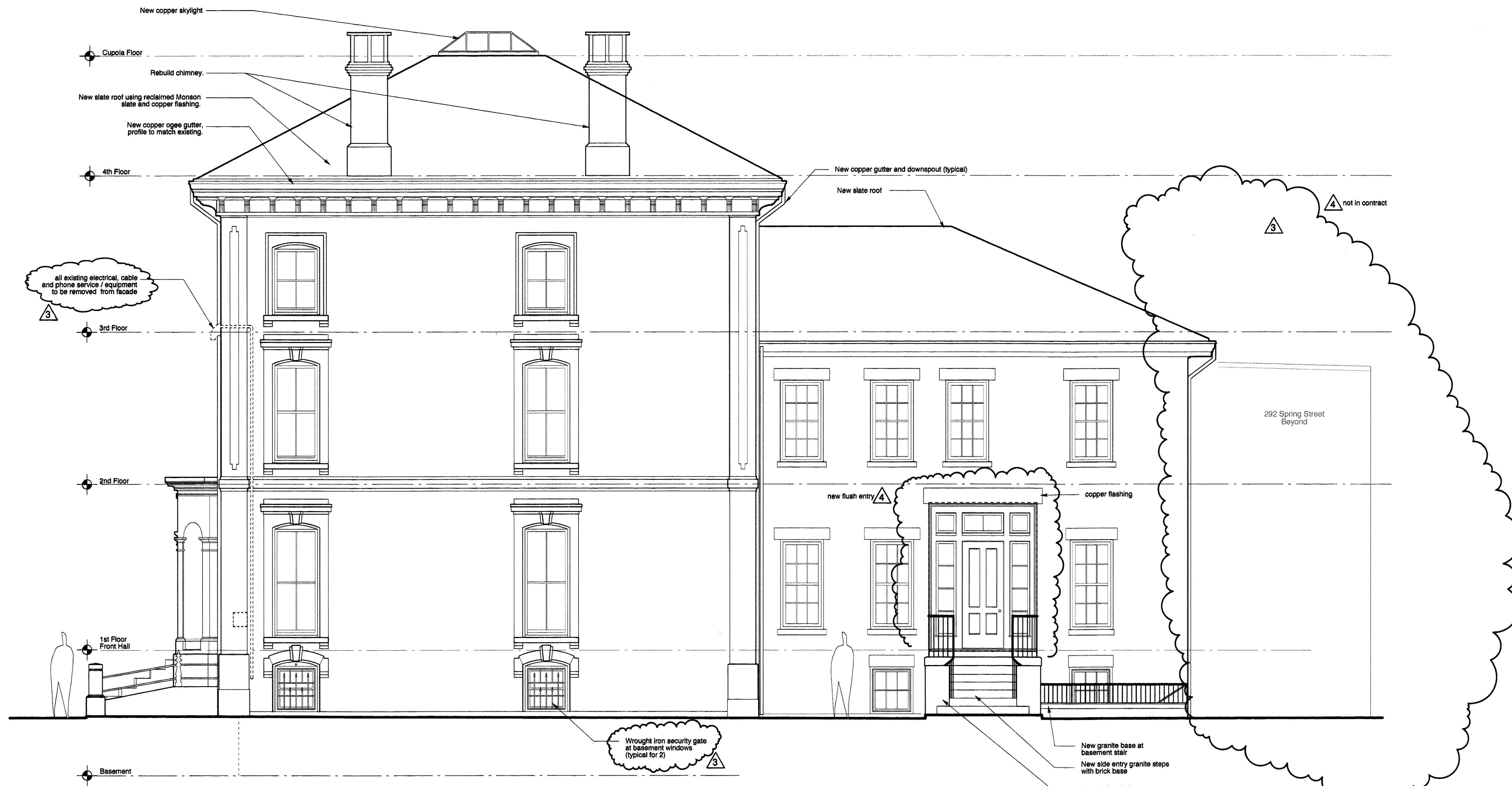
West Elevation SCALE: 1/4" = 1'-0"
