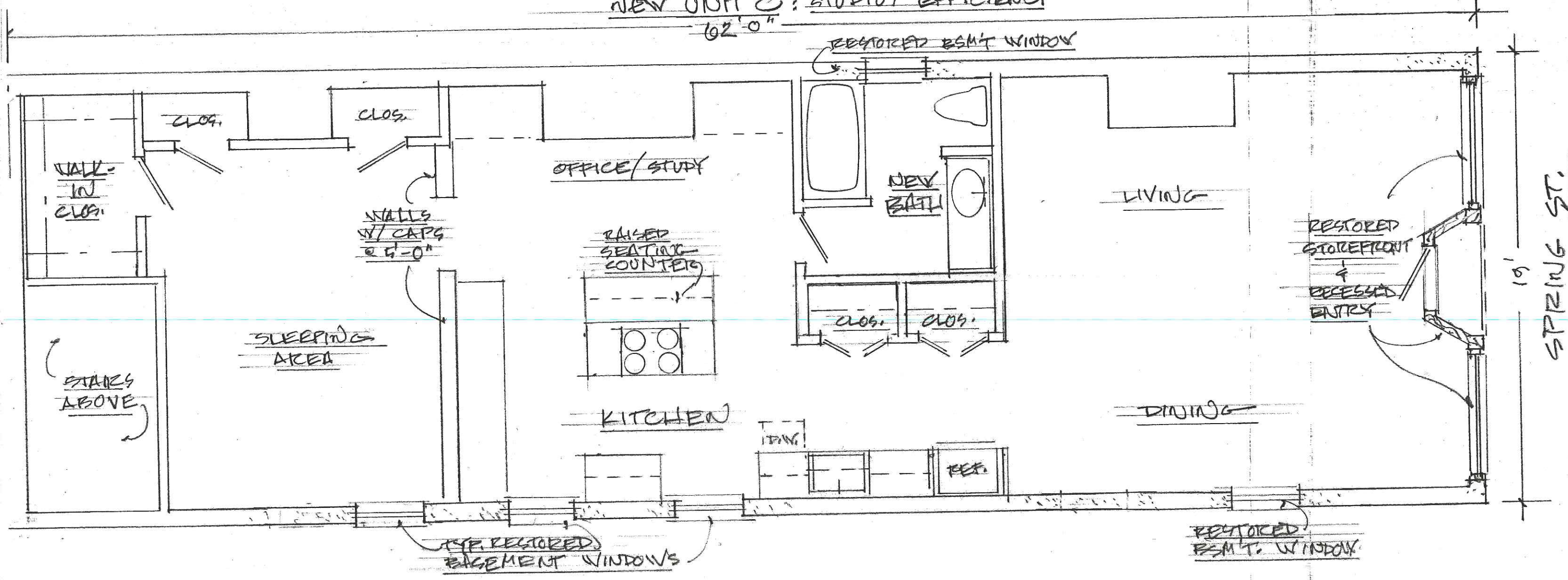
BASEMENT FLOOR PLAN - 249 SPRING ST. 1/4" = 1'-0" PROPOSED 6/12/17
