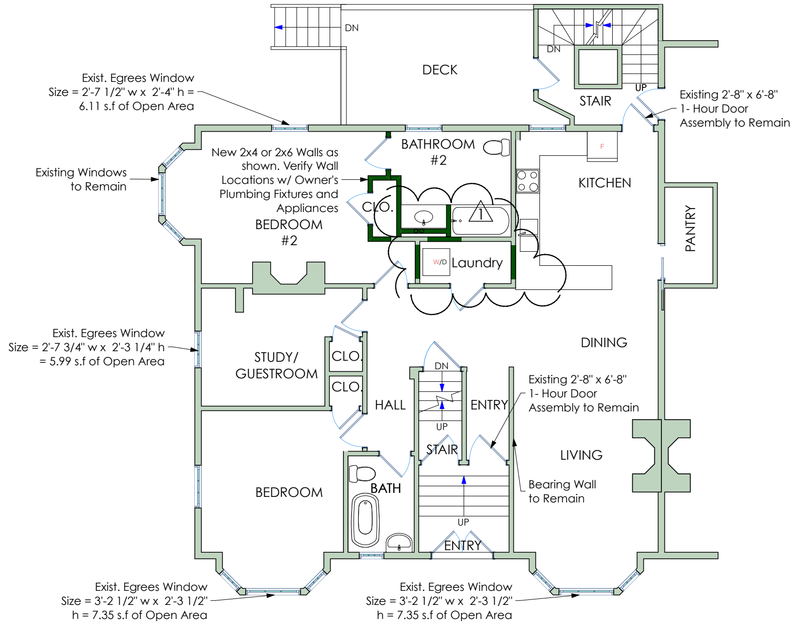
1 Proposed First Floor Plan SCALE: 1/8" = 1'-0"
